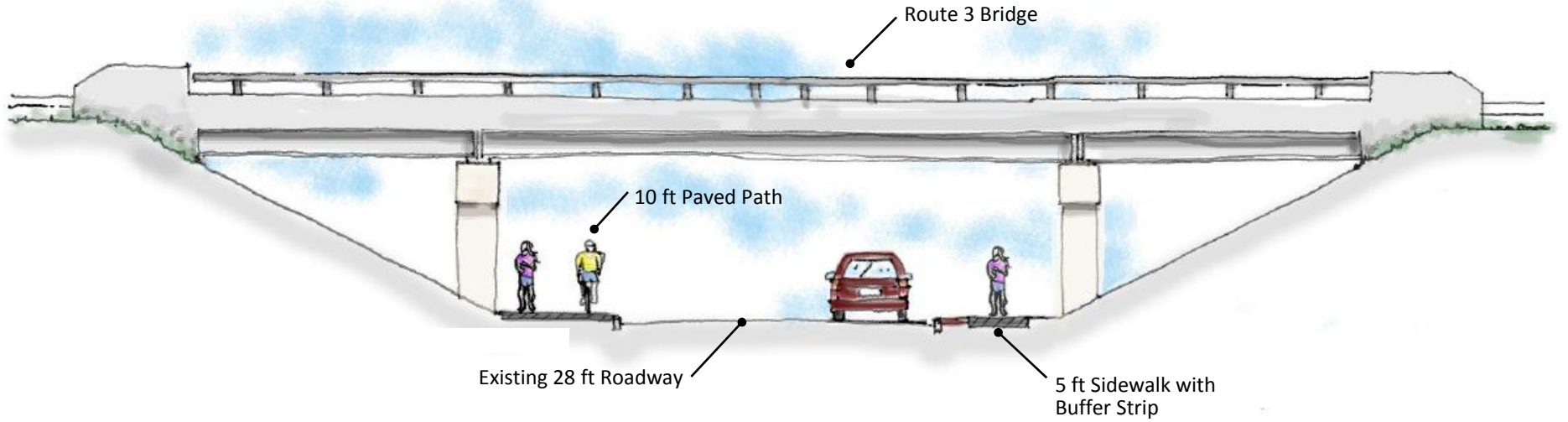
Naubuc Avenue | Section at Route 3 Underpass (looking northwest toward Putnam Boulevard)
