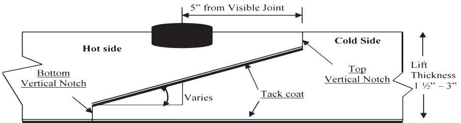
FIGURE 4.06-5: Notched Wedge Joint Cores (Not to Scale)
