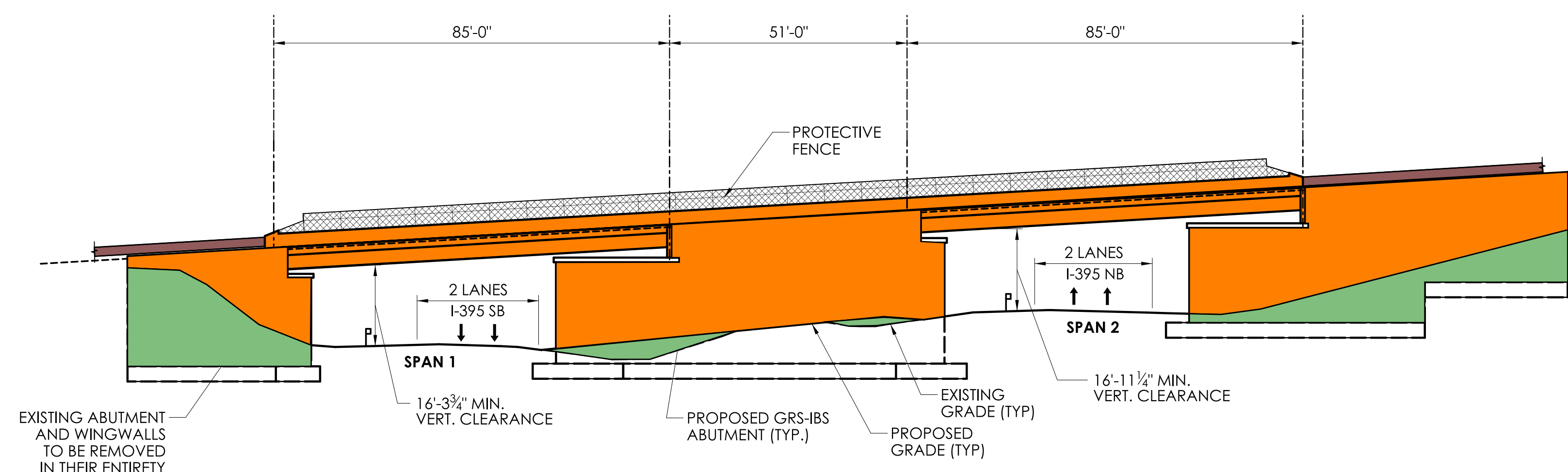
PROPOSED ELEVATION SCALE: 1" = 20'
