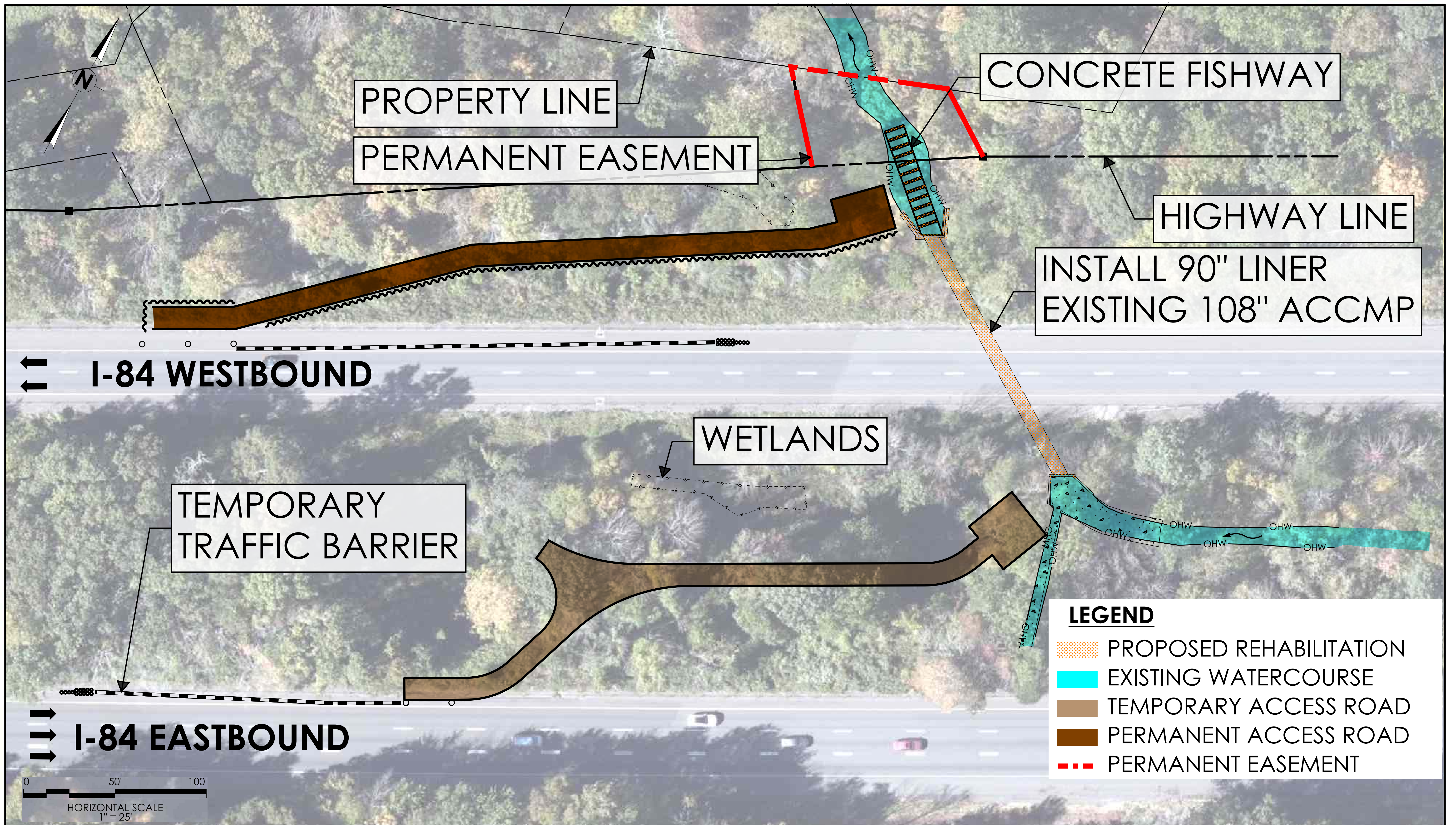
BRIDGE NO. 07042 - GENERAL PLAN INTERSTATE 84 WB OVER BULLET HILL BROOK SOUTHURY, CONNECTICUT
