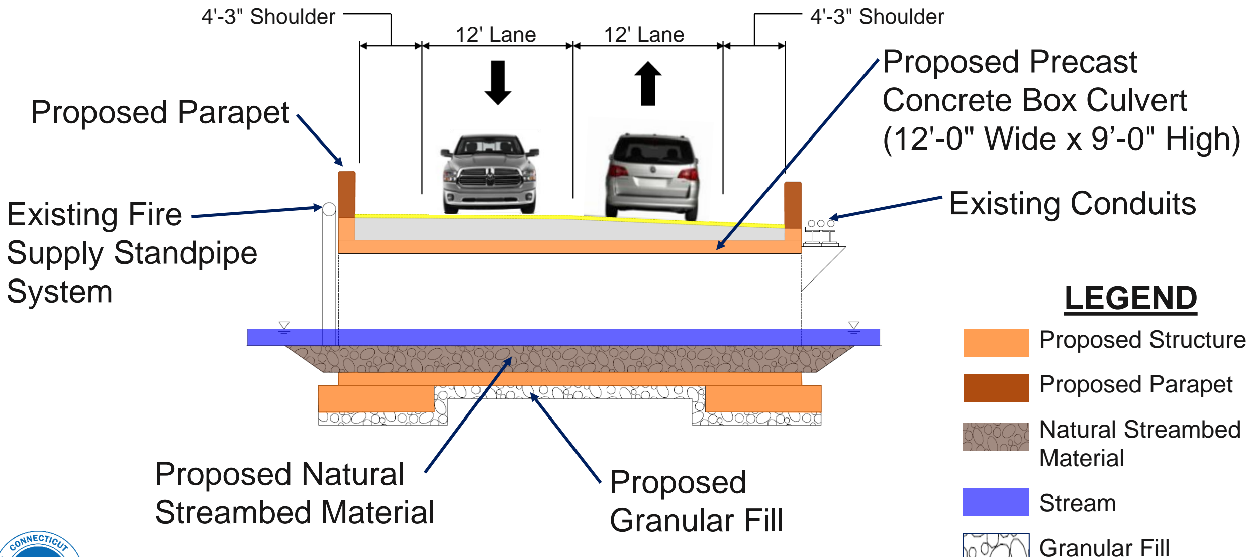
Section View of Proposed Structure
