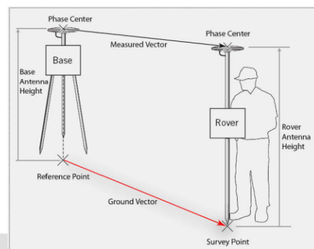
Figure 2-1 Typical RTK Setup.
