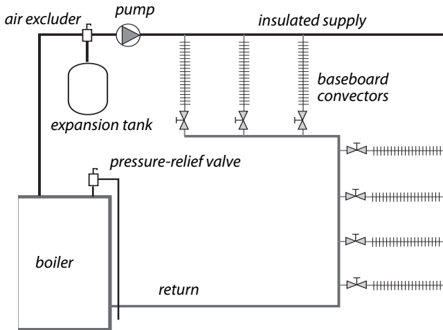
Simple reverse-return hot-water system: The reverse-return method of piping is the simplest way of balancing flow among the heat emitters.
