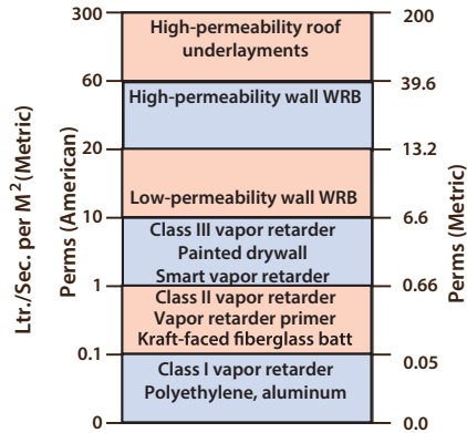
Vapor Permeability of Materials and Assemblies
