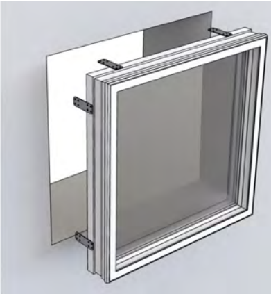
Block frame window installation: Block-frame windows don't have a fin. Installers use plates or screws to fasten the window to its opening.
