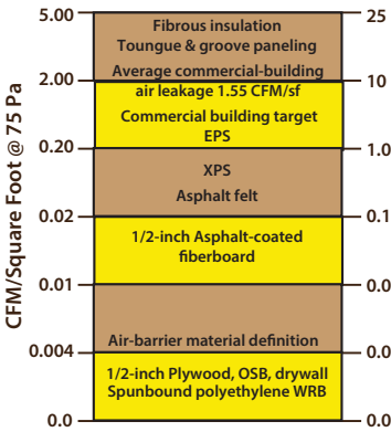
Air Permeability of Materials and Assemblies
