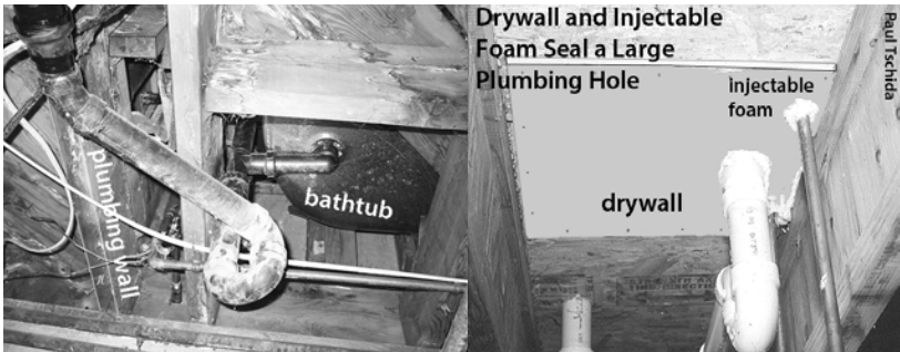
Sealing large plumbing penetrations: Bed drywall or wood sheathing in sealant and fasten with nails or screws. Fill gaps around the penetrations with one-part foam to complete this airtight seal.
