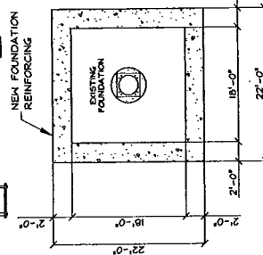
PLAN VIEW (FOUNDATION MODIFICATION)
