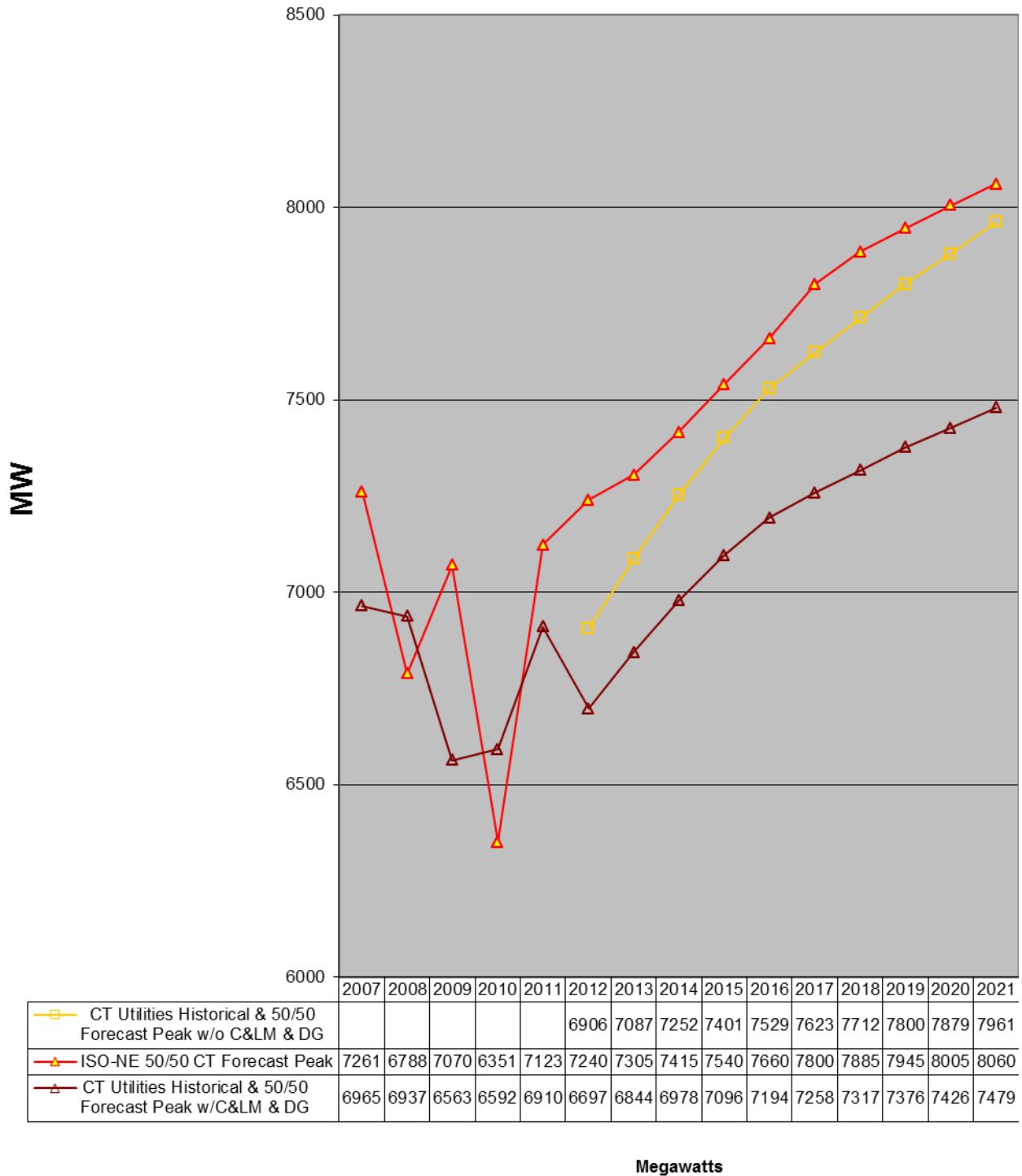
Figure 1b: 50/50 Forecasts in MW
