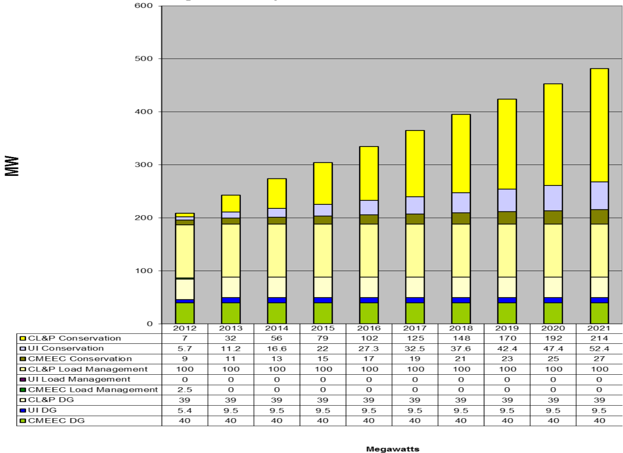
Figure 3: Load Reductions Due to Conservation, Load Management/Response, and Distributed Generation
