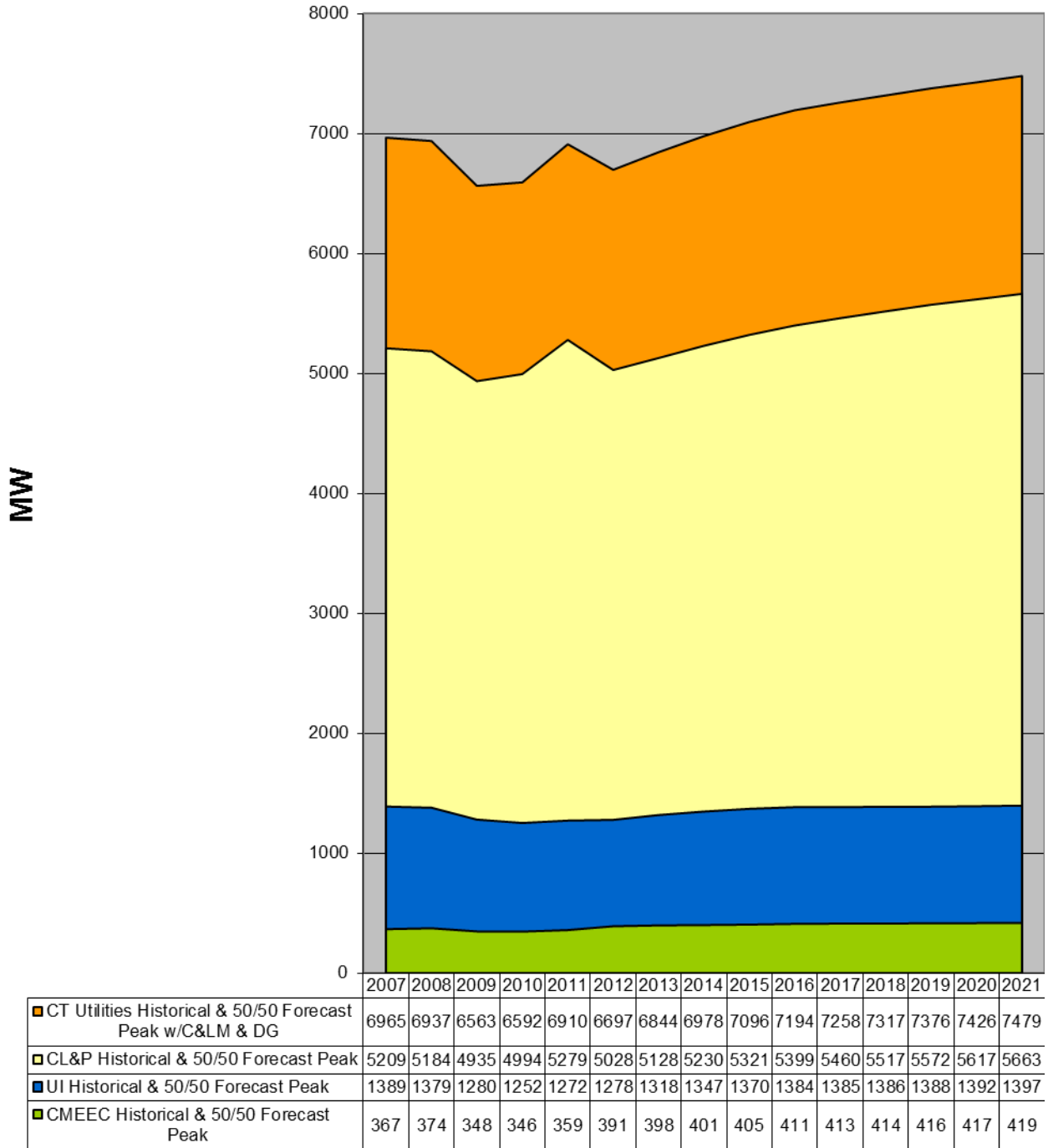
Figure 1a: Utility Adjusted Historical & 50/50 Peak Load Forecast in MW
