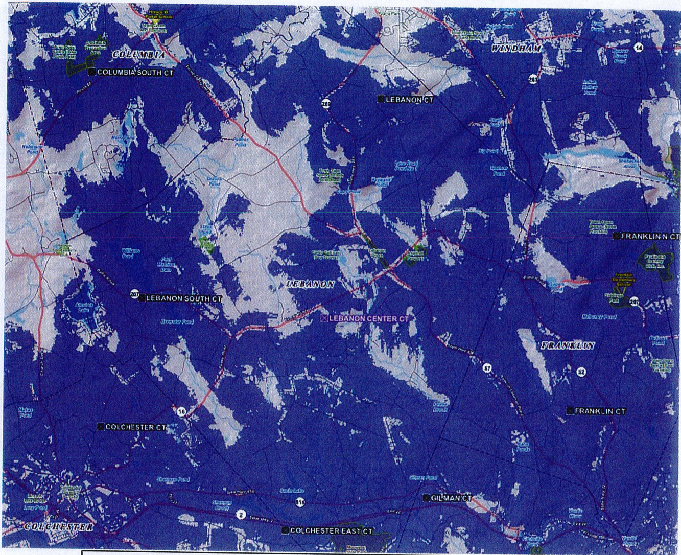
Figure 2 - Existing LTE 700 MHz Service
