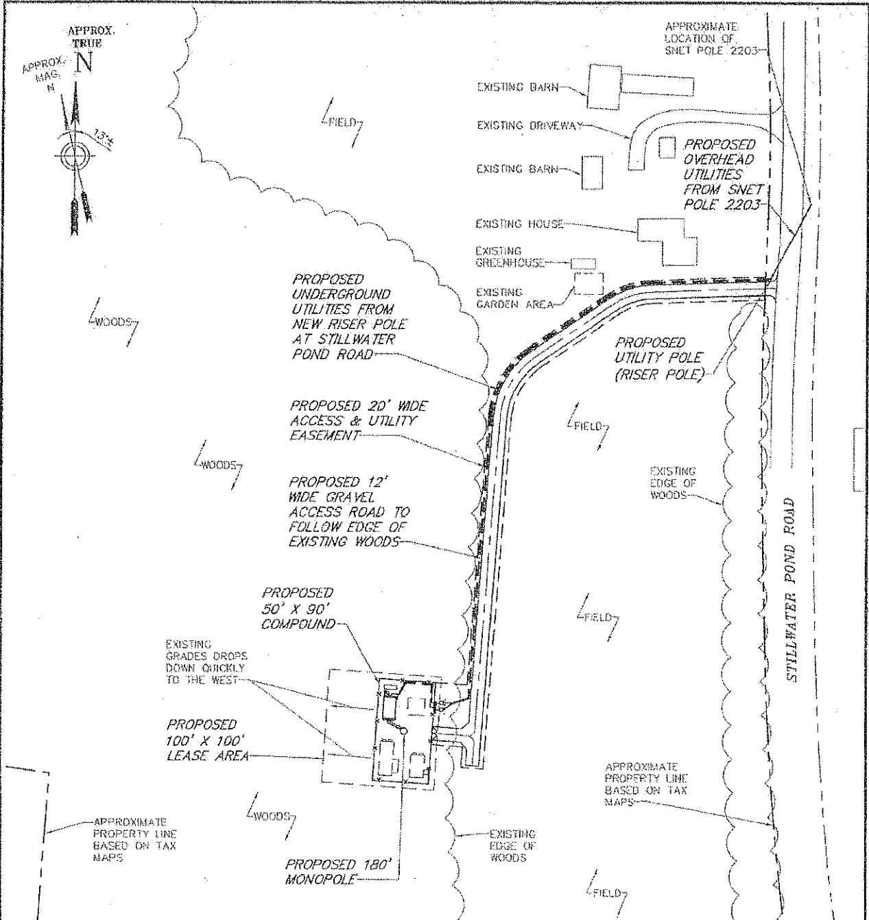
SITE PLAN GRAPHIC SCALE
