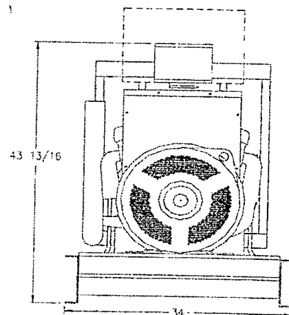
Drawing above for illustration purposes only, based on standard open power 480 volt generator. Lengths may vary with other voltages.
