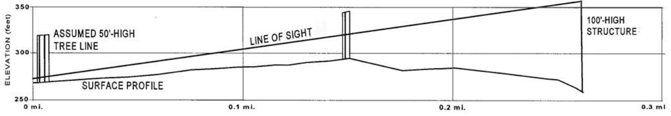
PROFILE 4: MANSFIELD NEW CEMETERY TO STRUCTURE 9077
