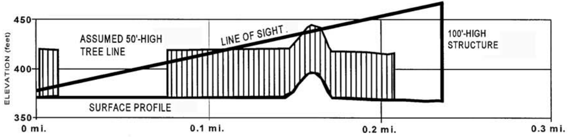
PROFILE 10: MUNYAN CEMETERY TO STRUCTURE 9316
