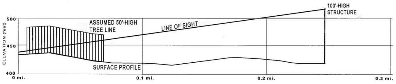
PROFILE 6: CHEWINK CEMETERY TO STRUCTURE 9110
