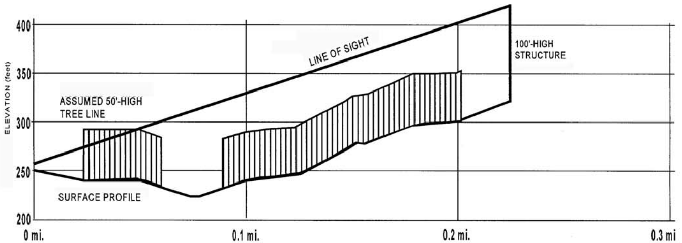
PROFILE 9: ROGERS VILLAGE TO STRUCTURE 9232
