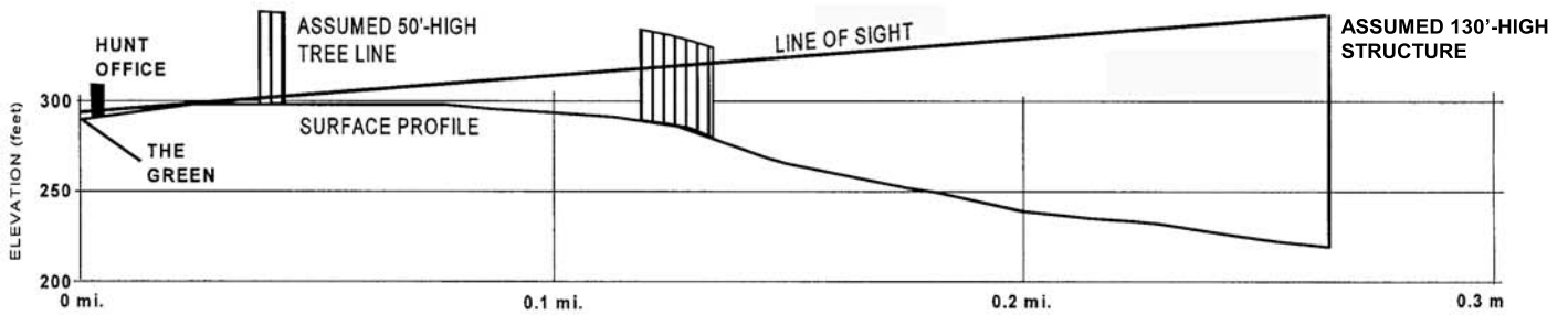
PROFILE 11: DR. CHESTER HUNT OFFICE TO WILLIMANTIC SOUTH OVERHEAD VARIATION
