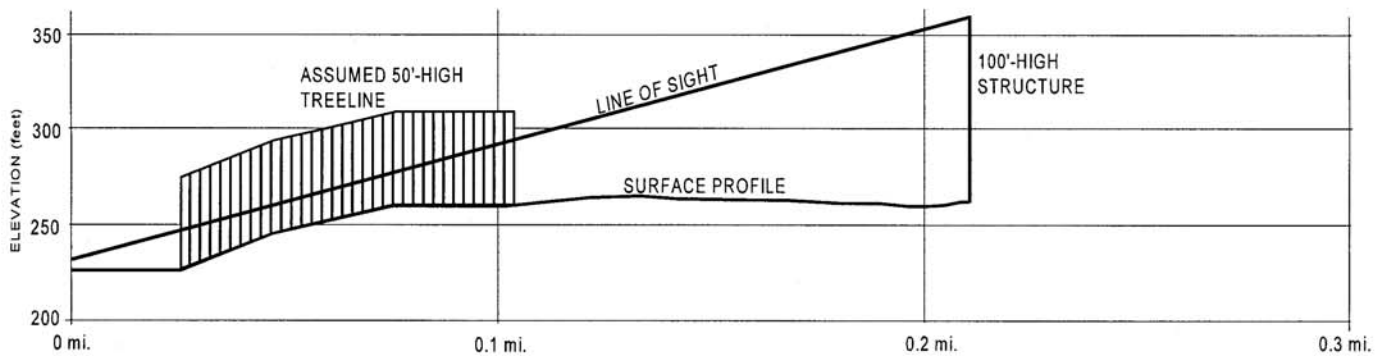
PROFILE 3: 89 MANSFIELD HOLLOW ROAD TO STRUCTURE 9075
