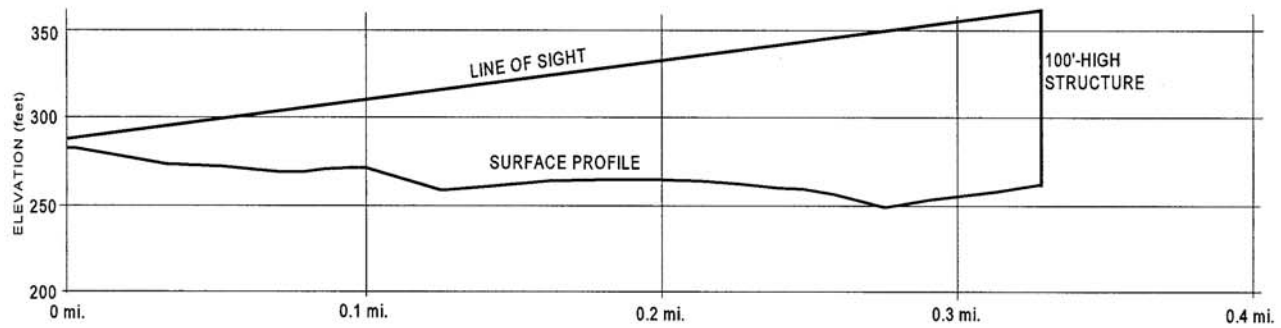
PROFILE 5: MANSFIELD OLD CEMETERY TO STRUCTURE 9076
