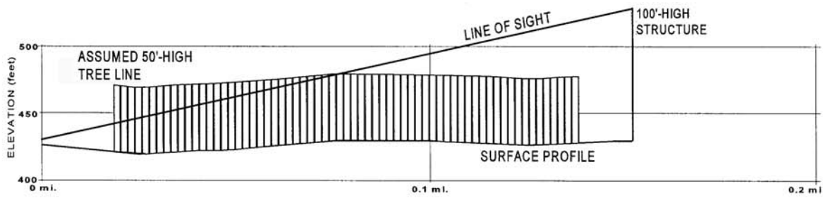
PROFILE 7: CHAPLIN OLD CEMETERY TO STRUCTURE 9112
