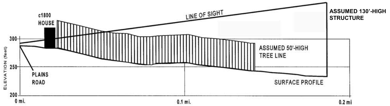
PROFILE 13: c1800 HOUSE TO WILLIMANTIC SOUTH OVERHEAD VARIATION
