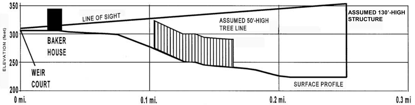
PROFILE 14: BAKER HOUSE TO WILLIMANTIC SOUTH OVERHEAD VARIATION
