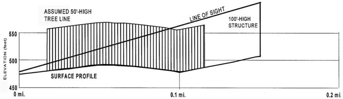
PROFILE 8: HAMPTON SOUTH CEMETERY TO STRUCTURE 9140
