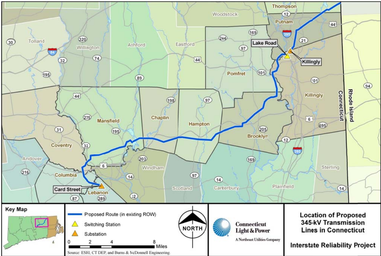
Figure 1-1 General Location of Connecticut Portion of the Proposed Interstate Reliability Project
