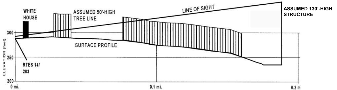
PROFILE 12: ELISHA WHITE HOUSE TO WILLIMANTIC SOUTH OVERHEAD VARIATION
