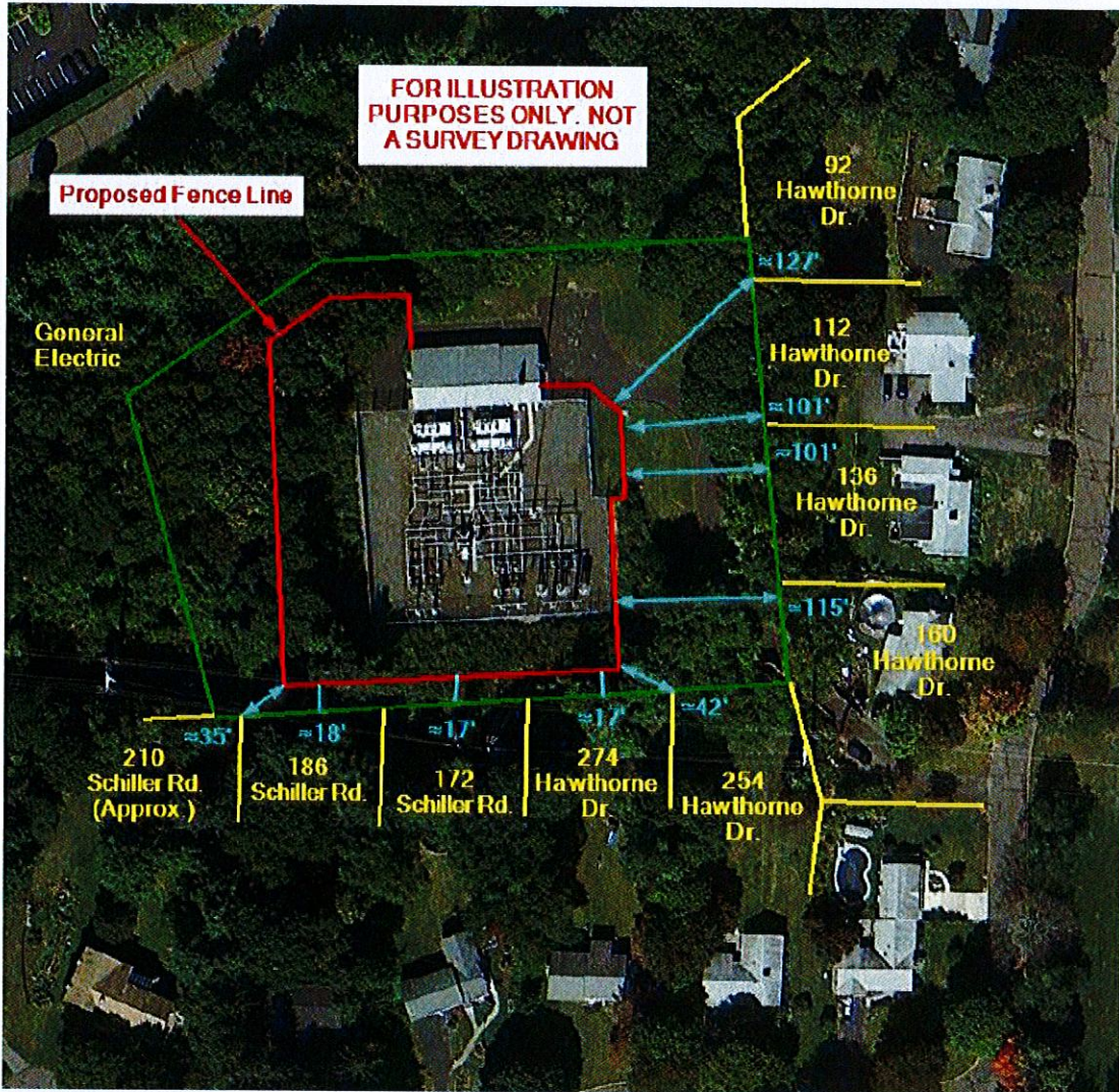
Figure 2: Proposed expansion area of Hawthorne Substation. Distances to abutting residences from initial proposed fence line shown - UI would increase the distance of the proposed fence to the south abutting properties. (UI 13, R. 11)
