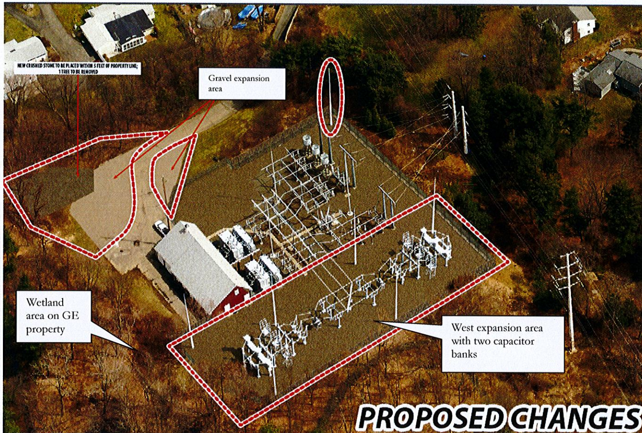
Figure 3: Photosimulation of proposed modifications. (UI 3) (final fence alignment and redesigned lightning mast protection system not shown)
