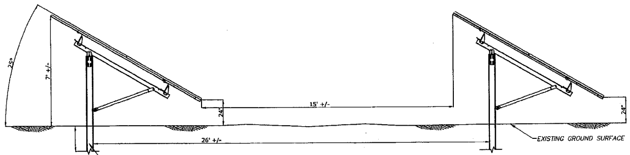
Figure 2 – Proposed Solar Rack Side Elevation View
