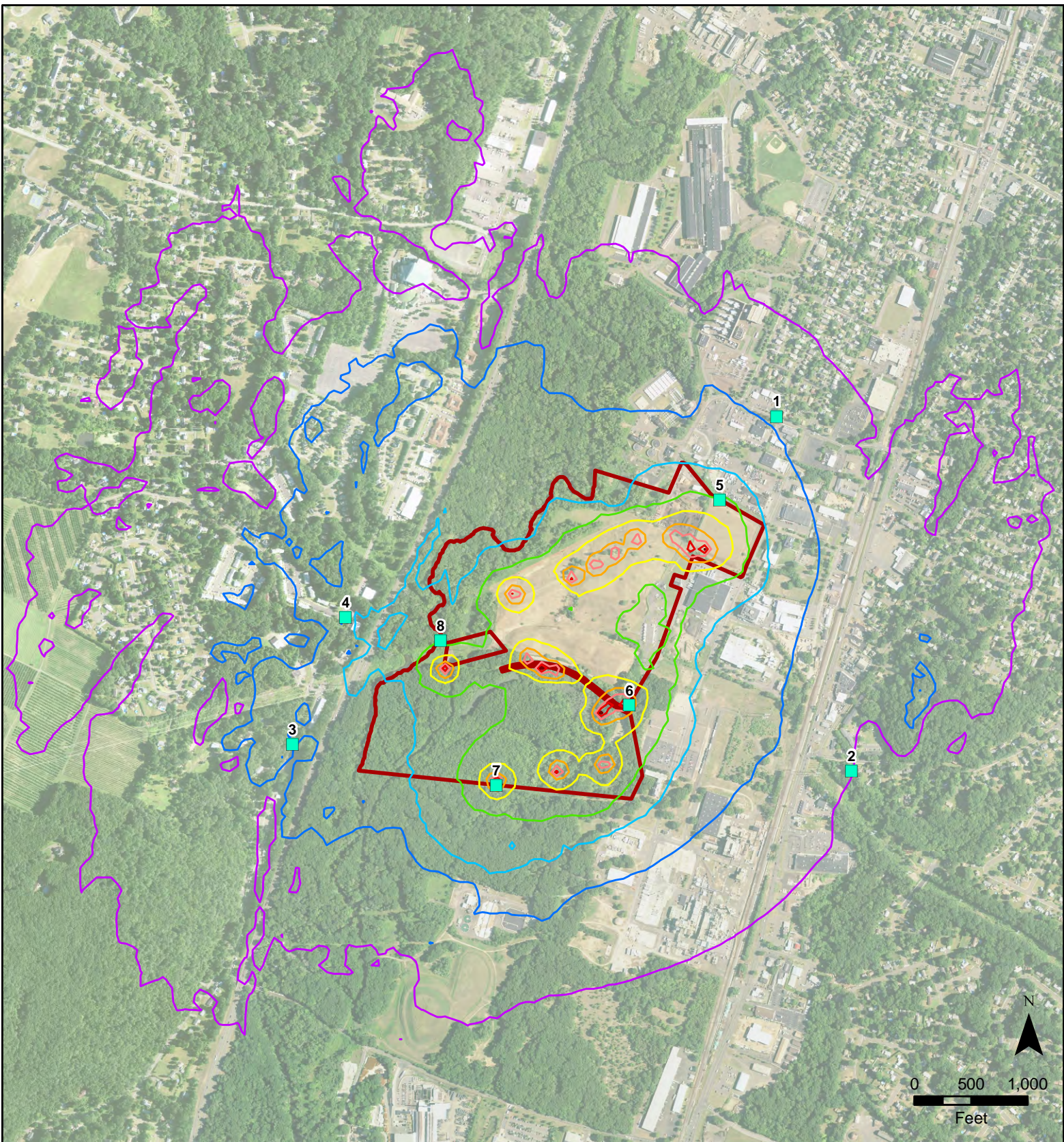
Figure 16 Sound Level Contours
