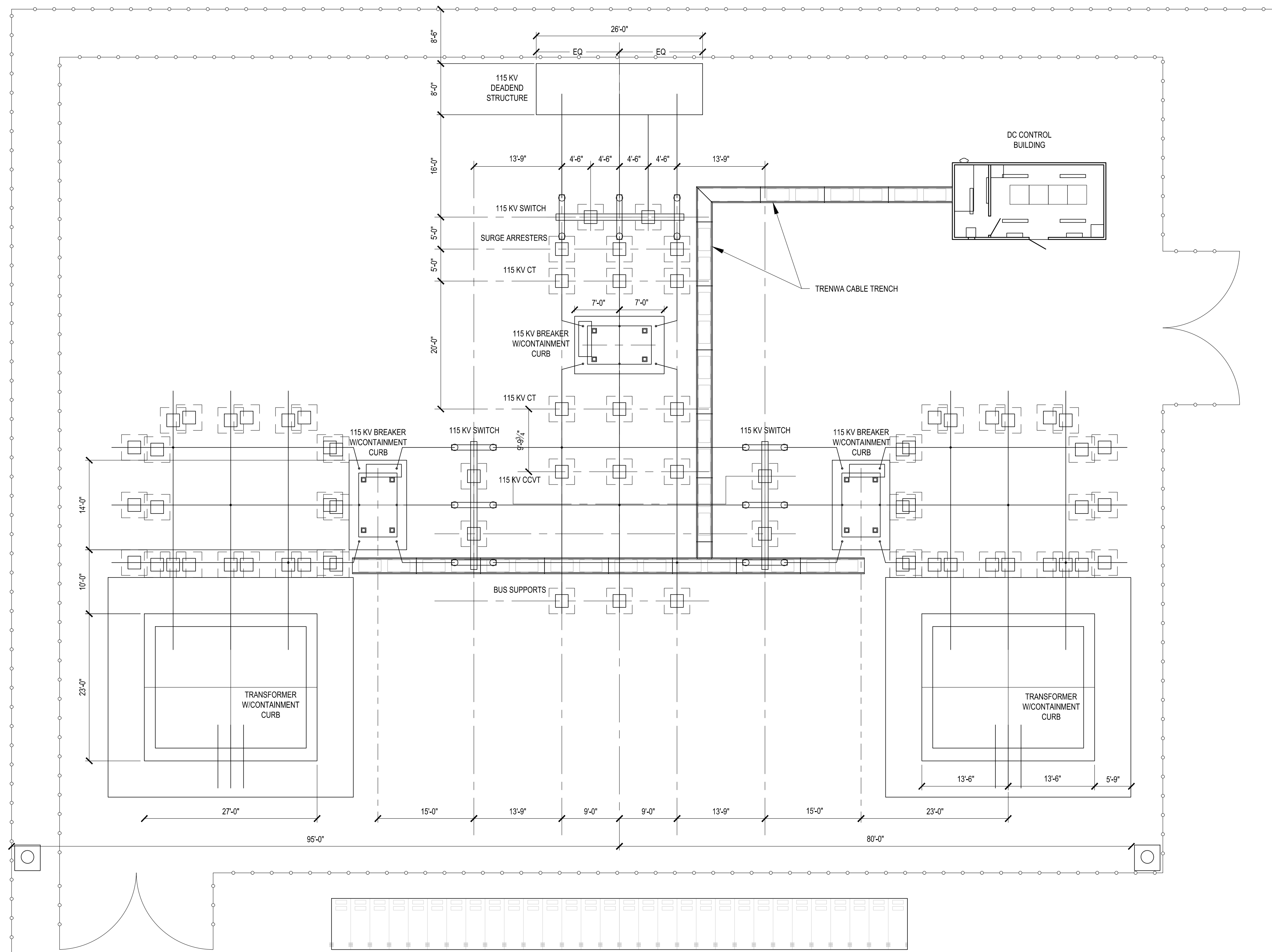
1 ENLARGED PLAN SCALE: 1" = 10'-0" SWITCHYARD ELECTRICAL LAYOUT
