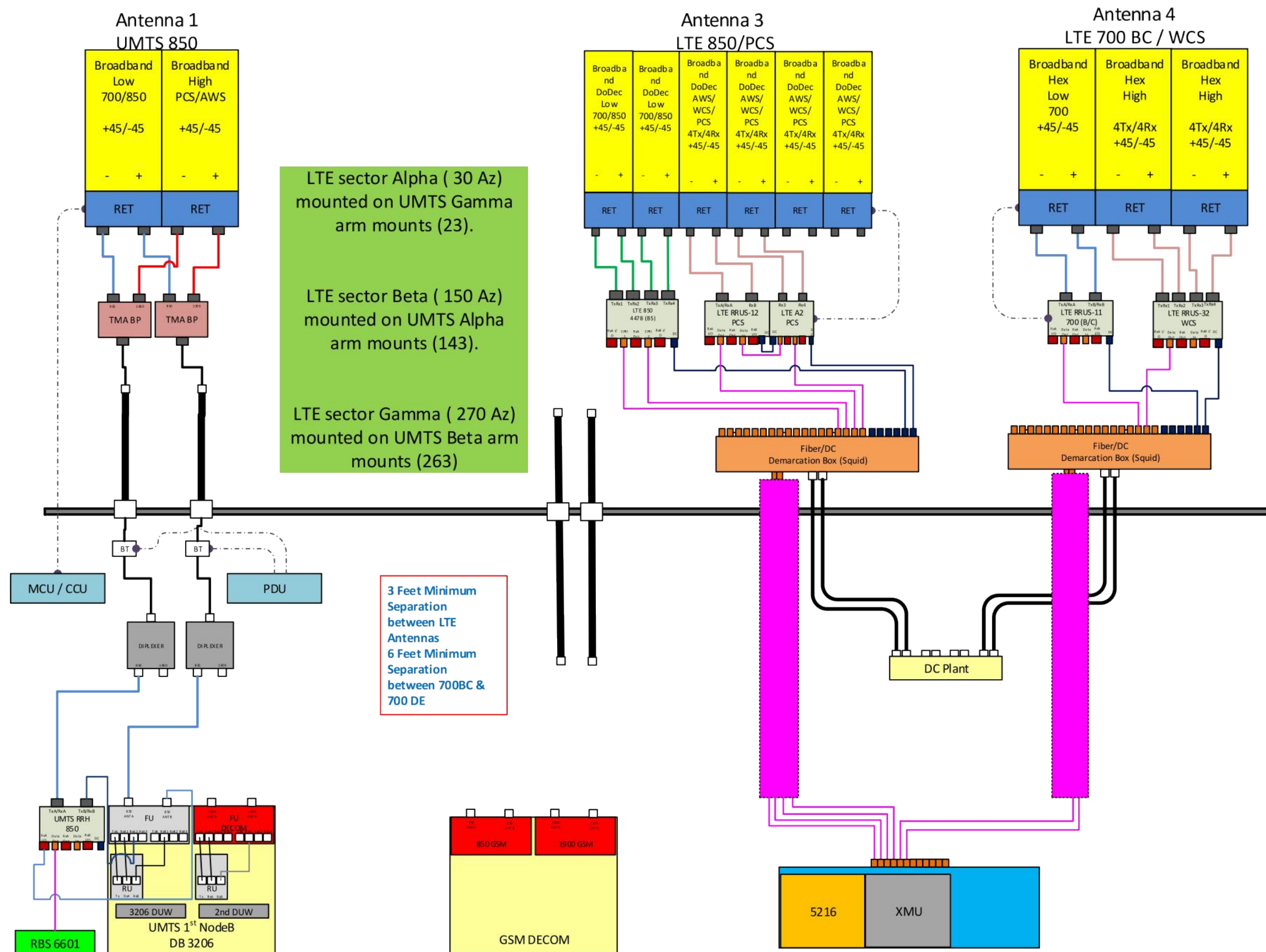
5 RF PLUMBING DIAGRAM E-3 NOT TO SCALE
