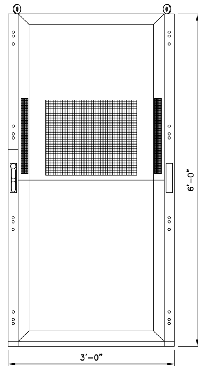
FRONT VIEW
