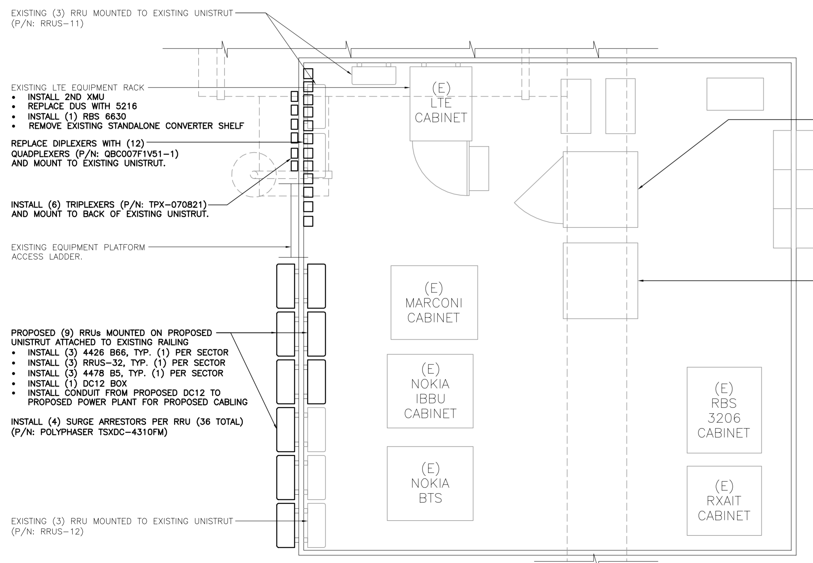
2 C-1 EQUIPMENT LAYOUT PLAN SCALE: 1/2" = 1' APPROXIMATE NORTH GRAPHIC SCALE ( IN FEET ) 1/2 inch = 1 ft.
