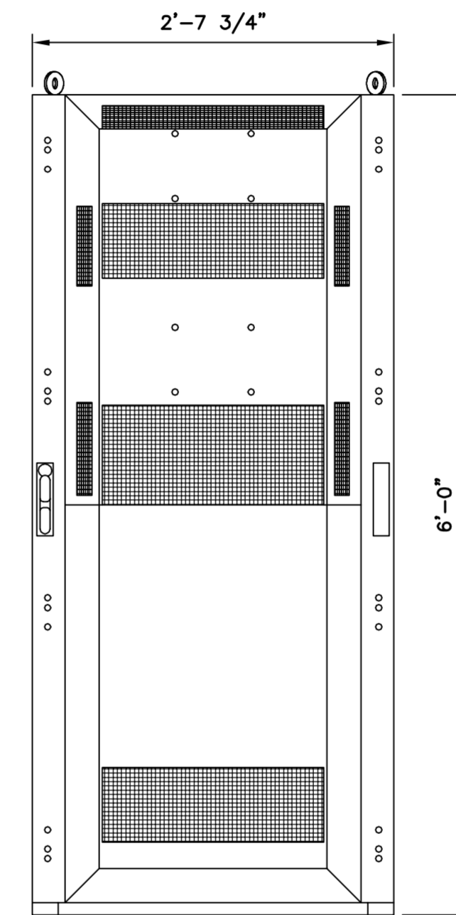
FRONT VIEW
