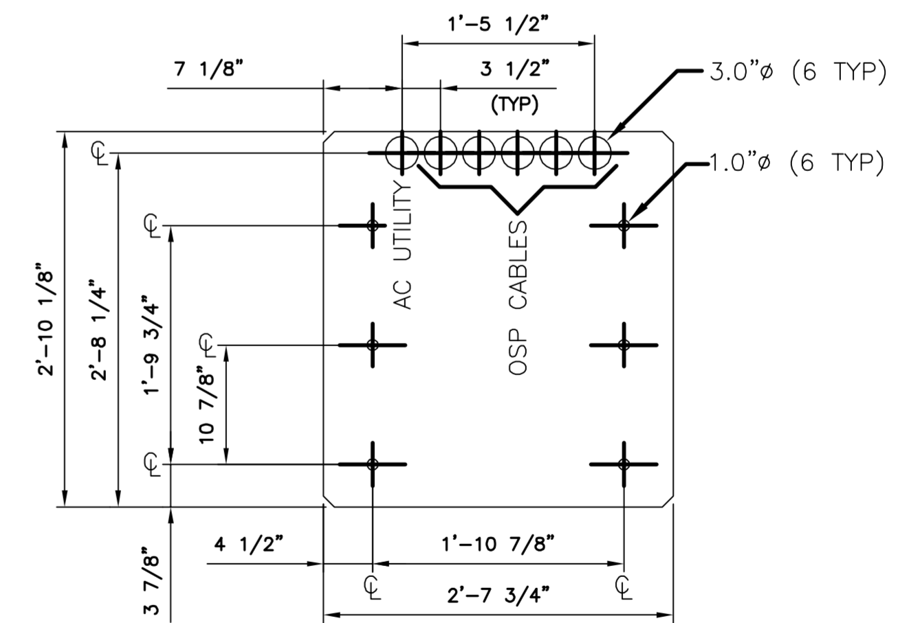
MOUNTING TEMPLATE
