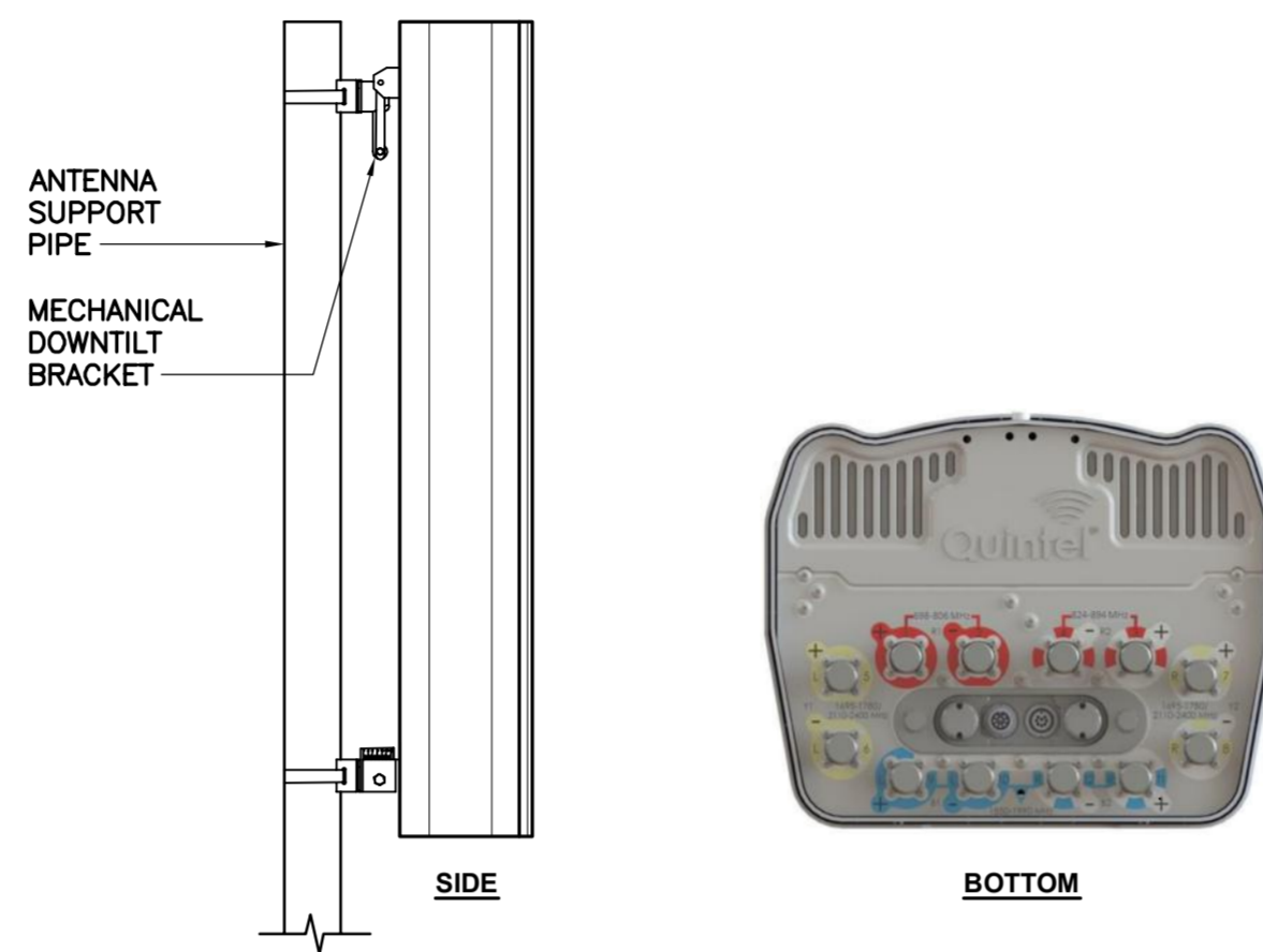
ALPHA/BETA/GAMMA ANTENNA
