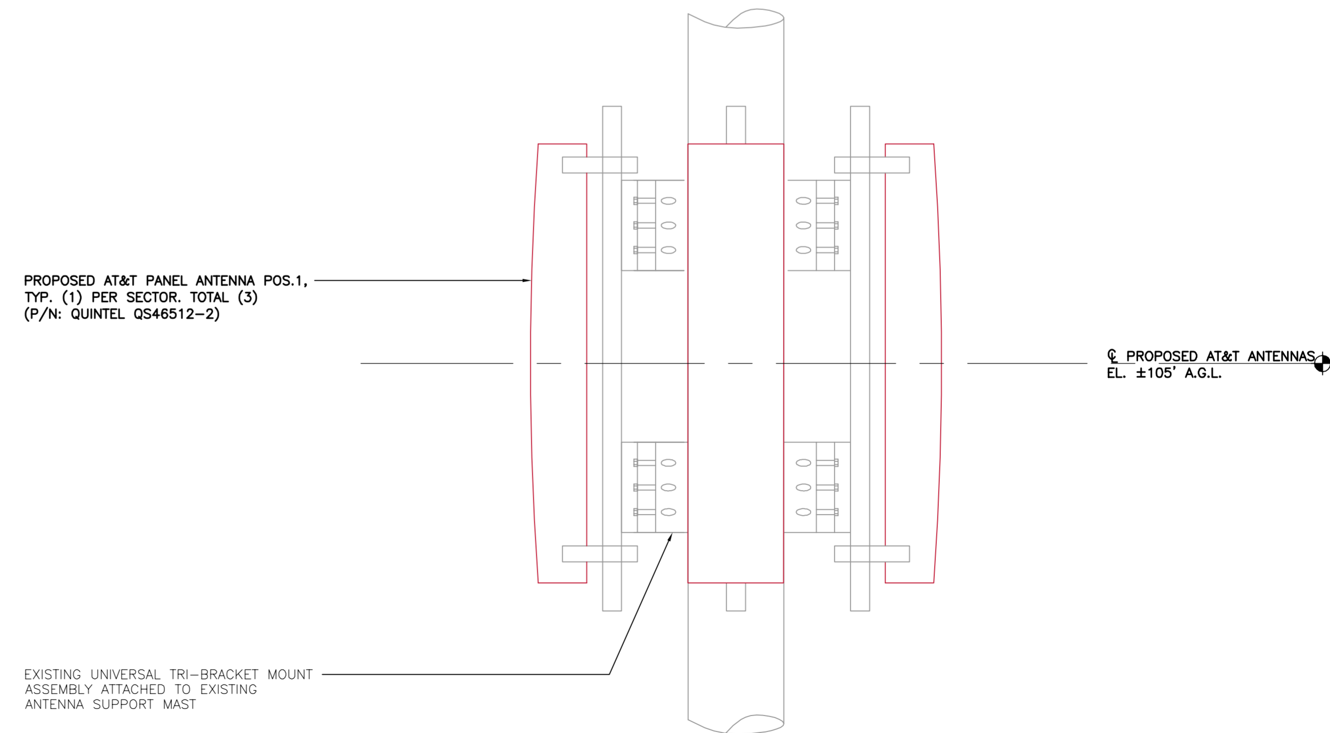
2A C-2 PROPOSED ANTENNA ELEVATION SCALE: 1" = 1'-0"
