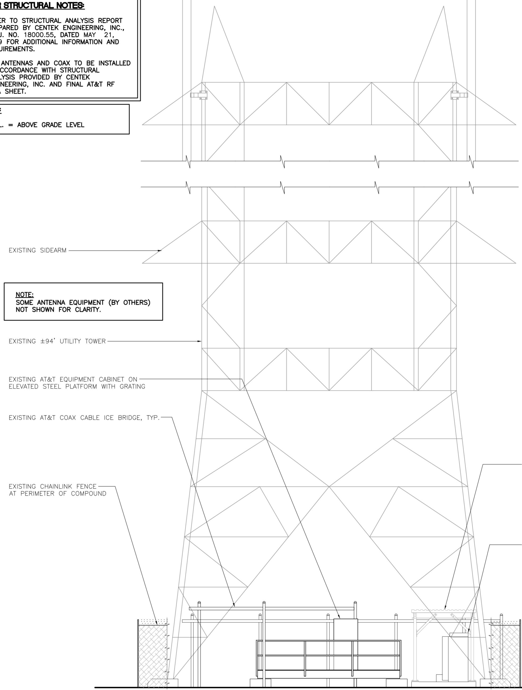
3 C-1 PARTIAL SOUTHWEST ELEVATION - PROPOSED SCALE: 3/16" = 1'-0"
