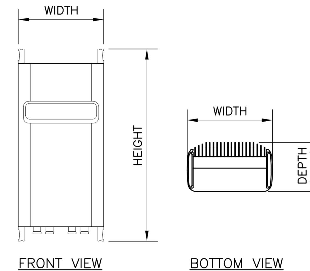
FRONT VIEW
