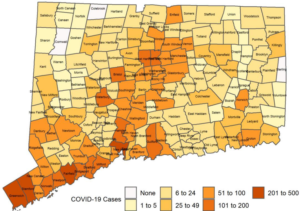
Number of COVID-19 Cases among People Living in Community Settings by Town with Specimen Collection or Onset Date During March 27 - April 09
