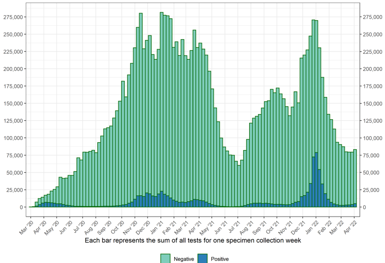
Number of Molecular Laboratory Tests for COVID-19 Reported via ELR Weekly test total by Specimen Collection Date As of April 13, 2022
