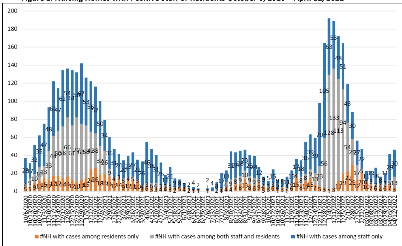
Figure 1. Nursing Homes with Positive Staff or Residents October 6, 2020 – April 12, 2022 1,2,3
