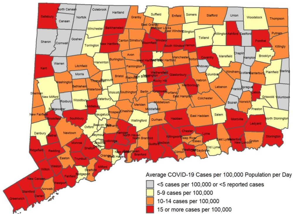
Average Daily Rate of COVID-19 Cases among People Living in Community Settings per 100,000 Population by Town with Specimen Collection or Onset Date During March 27 - April 09
