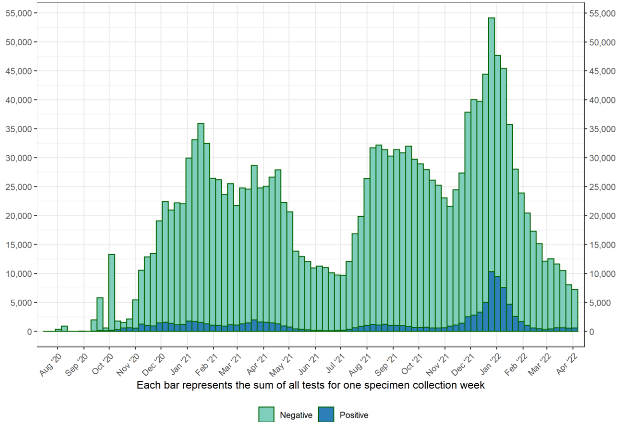
Number of Antigen Tests for COVID-19 Reported via ELR Weekly test total by Specimen Collection Date As of April 13, 2022
