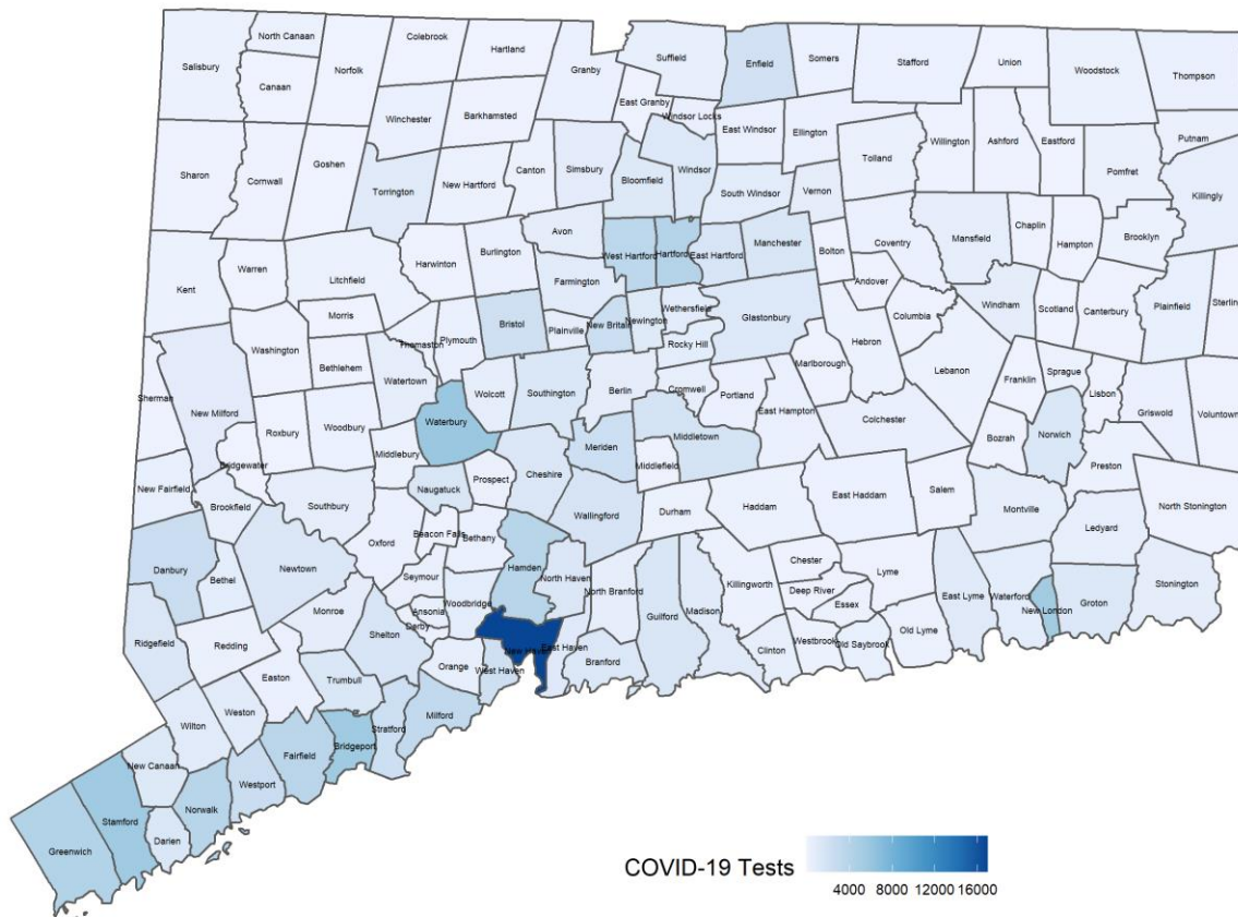
Number of Molecular and Antigen Tests for COVID-19 among People Living in Community Settings by Town with Specimen Collection Date During March 27 - April 09
