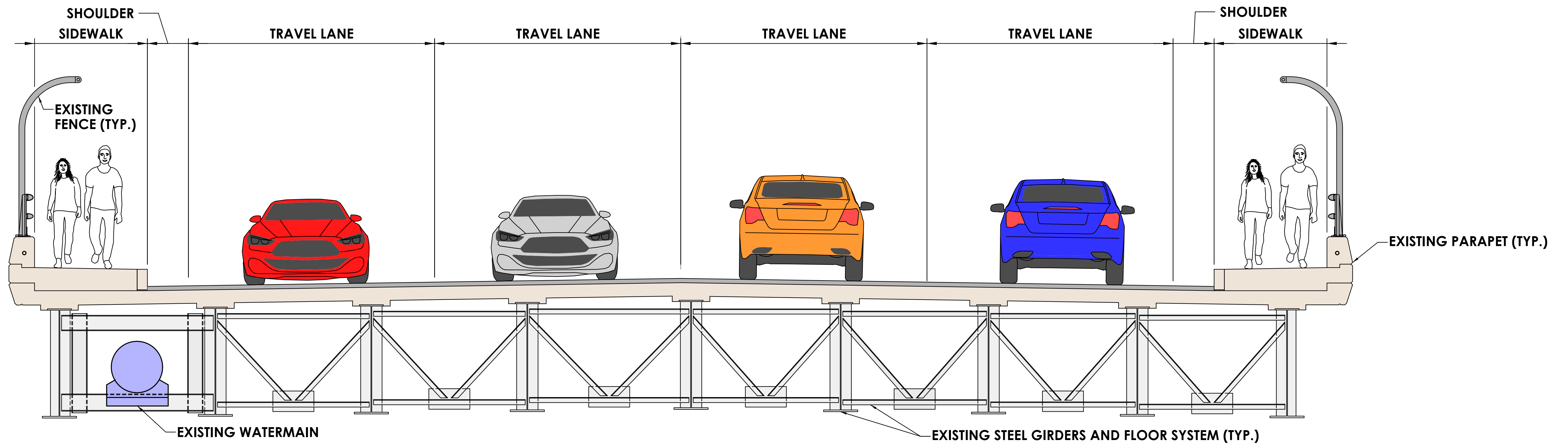
EXISTING SECTION
