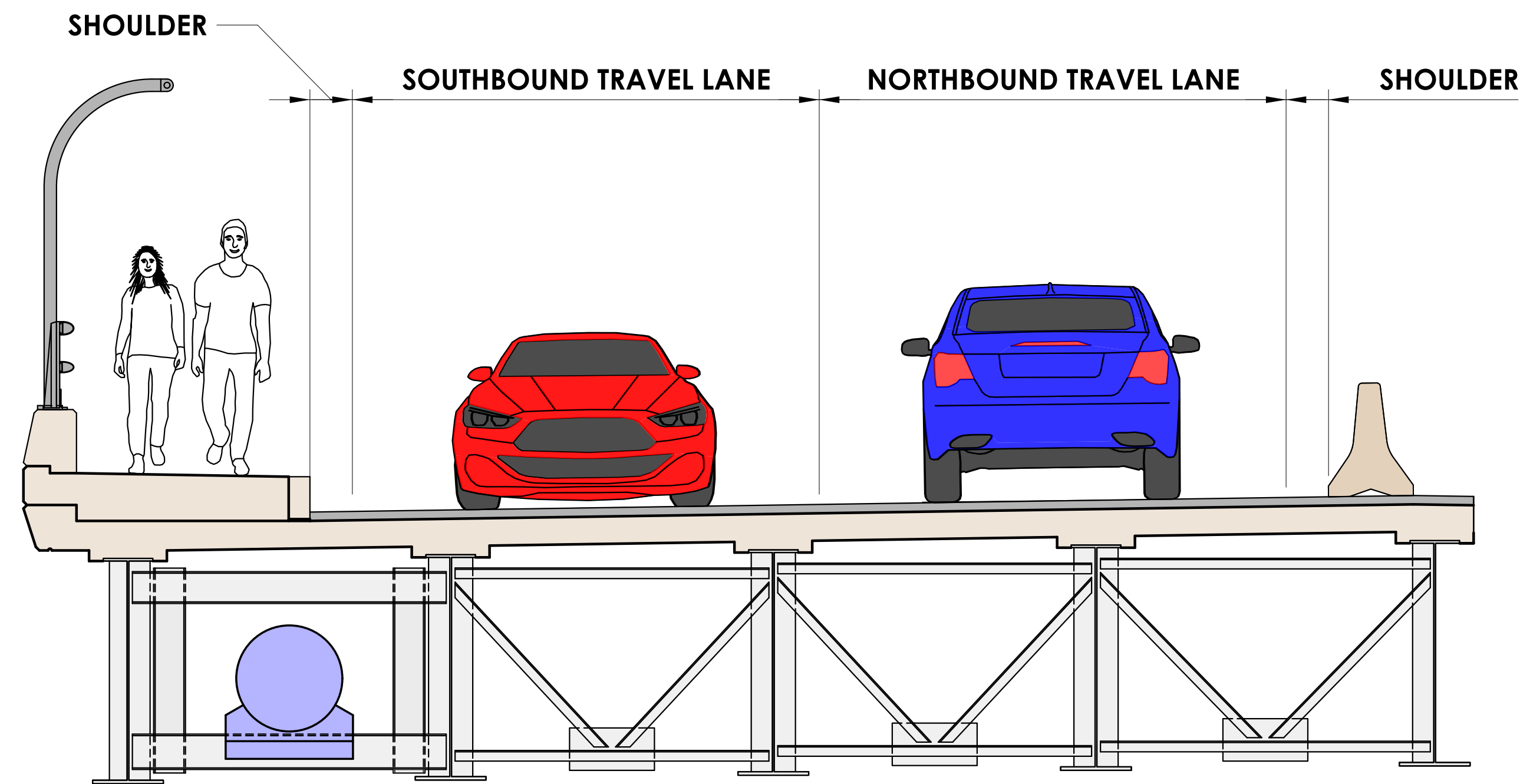
MAINTENANCE AND PROTECTION OF TRAFFIC STAGING PLAN - STAGE 1
