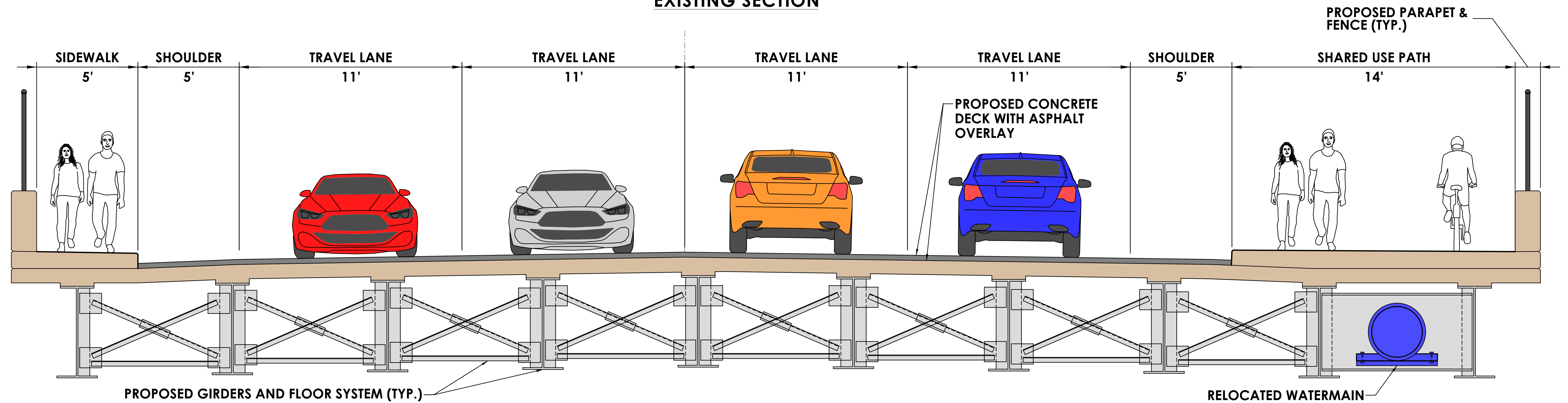
EXISTING SECTION
