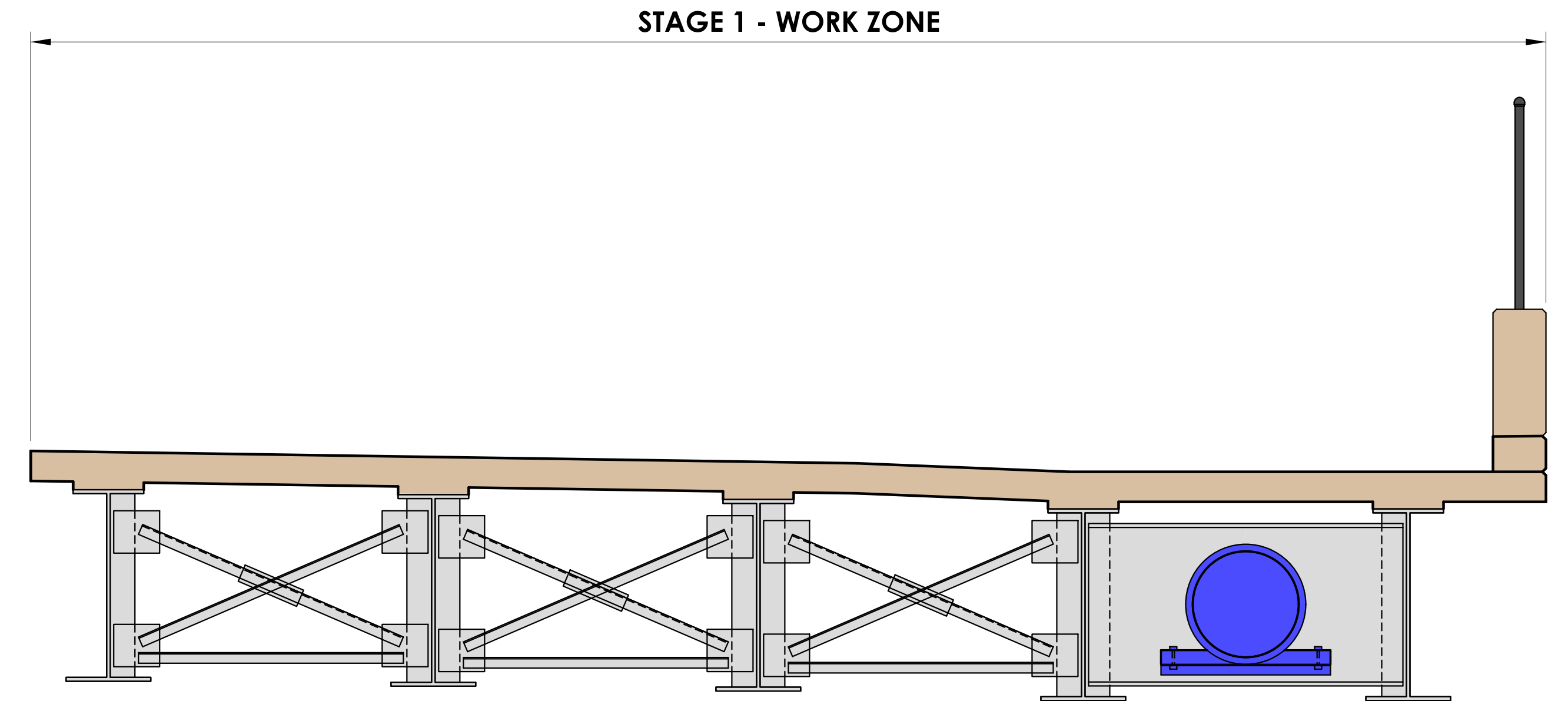
MAINTENANCE AND PROTECTION OF TRAFFIC STAGING PLAN - STAGE 1
