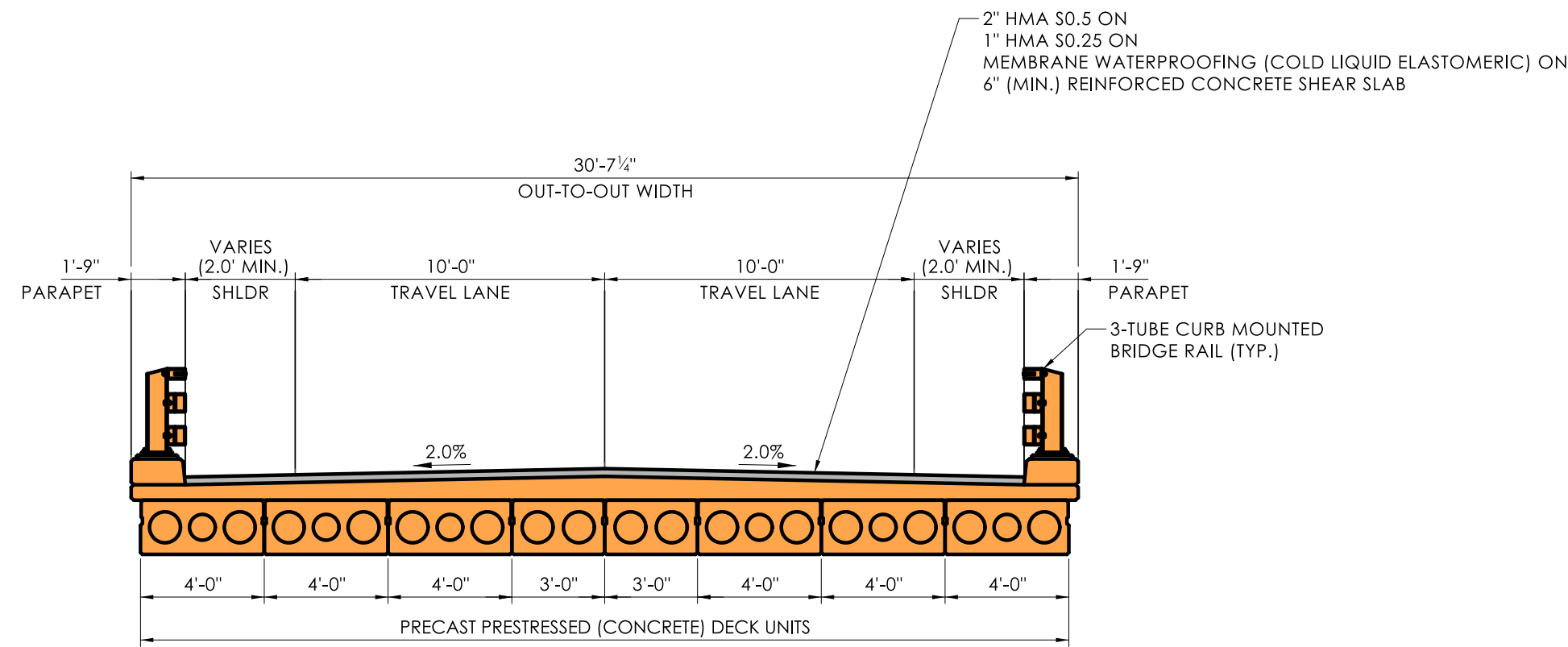
TYPICAL SECTION
