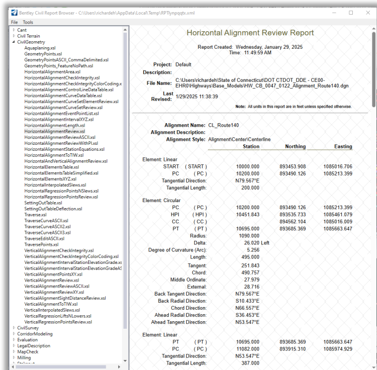
Figure 110 - Horizontal Geometry Report Output
