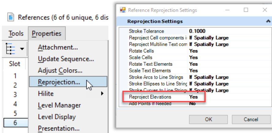
Figure 147 – Reproject Elevations
