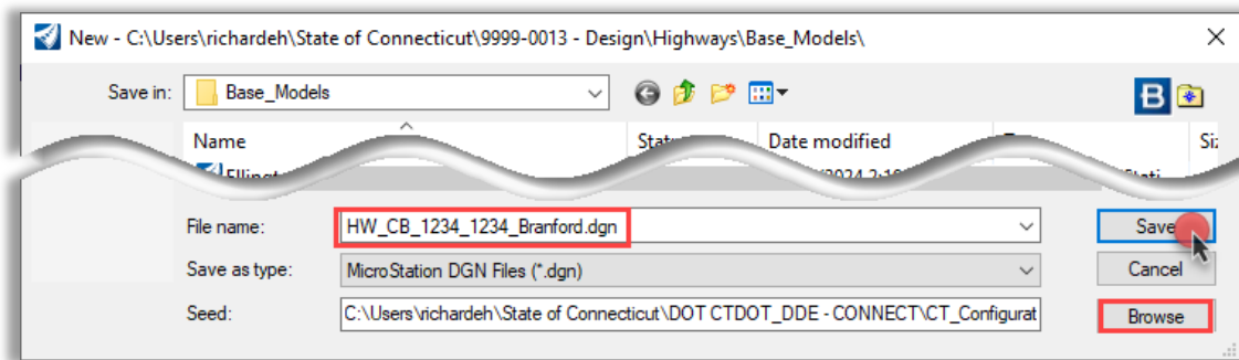
Figure 35- New File
