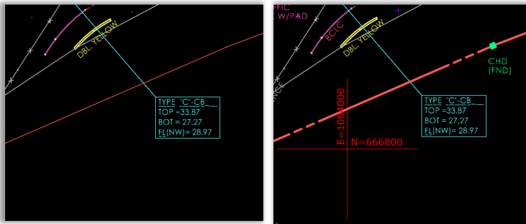
Figure 16 – Annotation Scale
