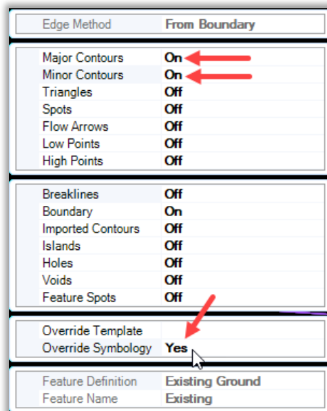
Figure 22 – Override Symbology
