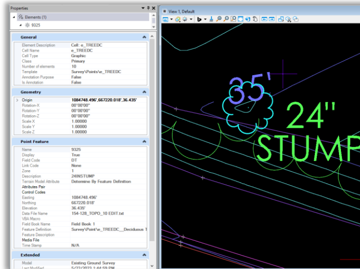
Figure 25 – Point Symbology
