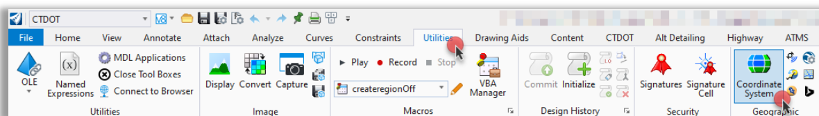
Figure 46 – Coordinate System
