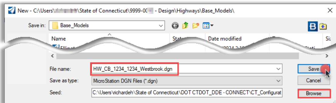
Figure 7 – New File
