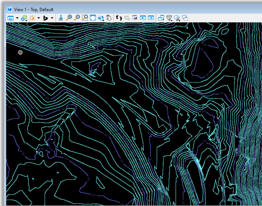
Figure 126 - Merge Terrain
