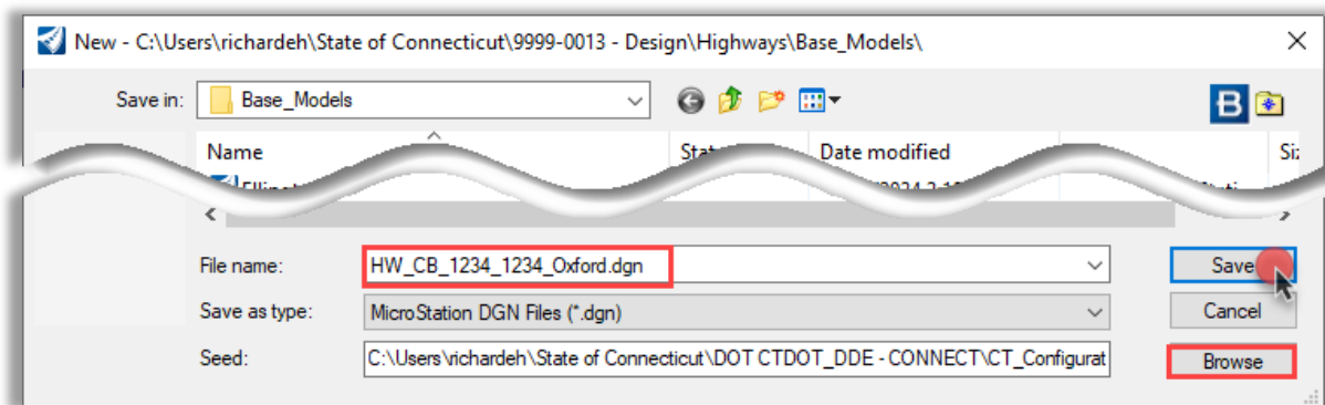
Figure 49 – New File
