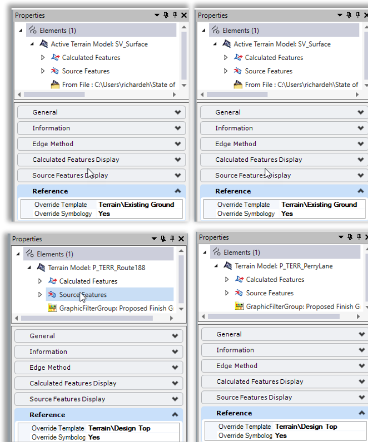
Figure 123 – Terrain Overrides
