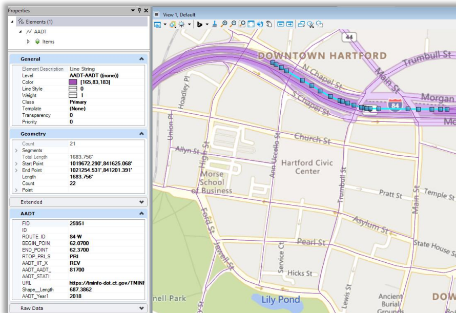
Figure 140 – AADT Properties
