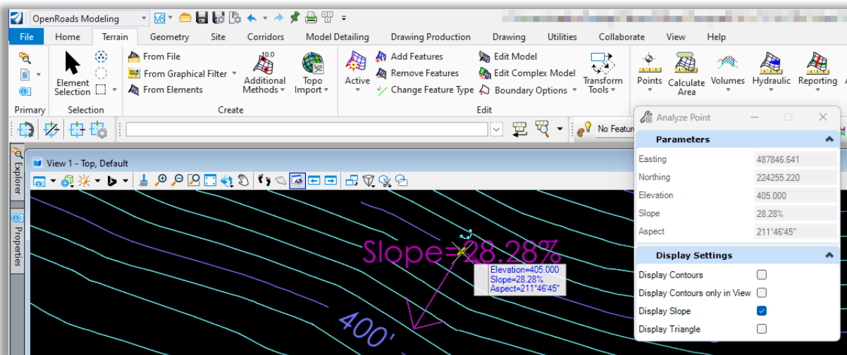
Figure 132 – Analyze Point
