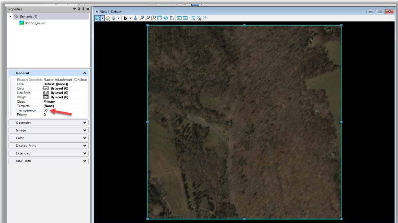
Figure 70 – Set Transparency
