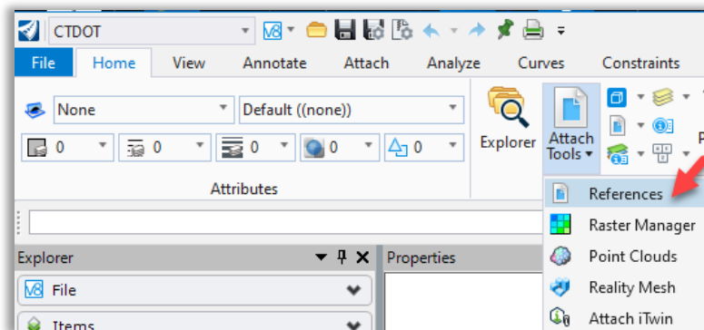
Figure 10 – References Tool
