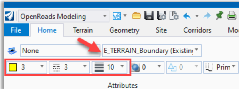
Figure 85 – Set Attributes
