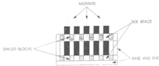
DIAGRAM OF A TYPICAL RACK
