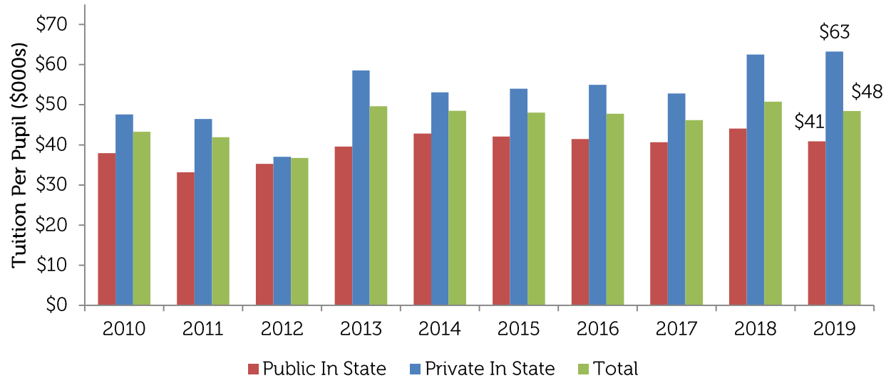
HPS Special Education Tuition Per Pupil ($000s)
