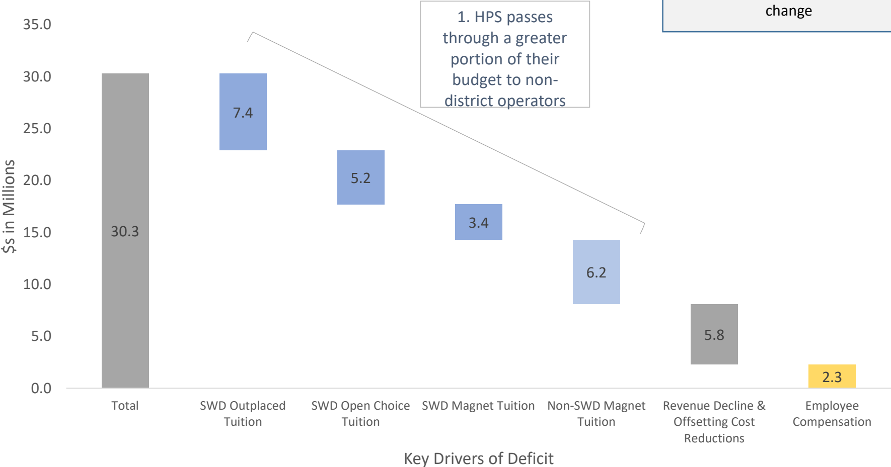
Summary of HPS Deficit Drivers
