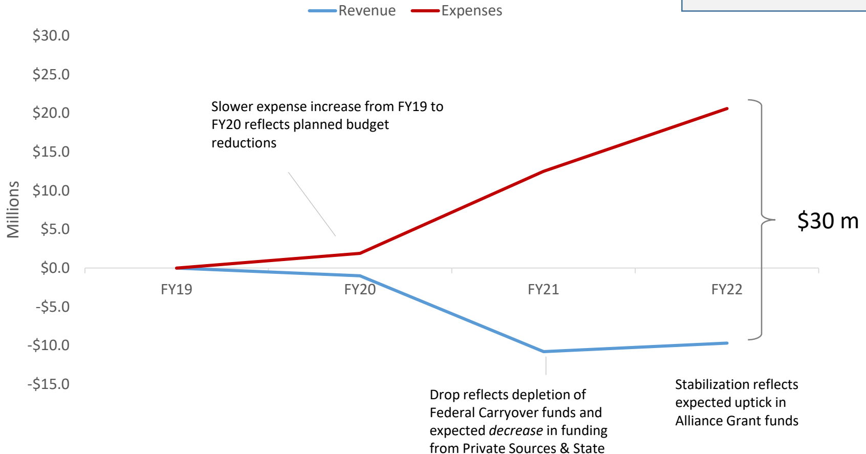
Projected Change in Revenue and Expenditures FY19-FY22
