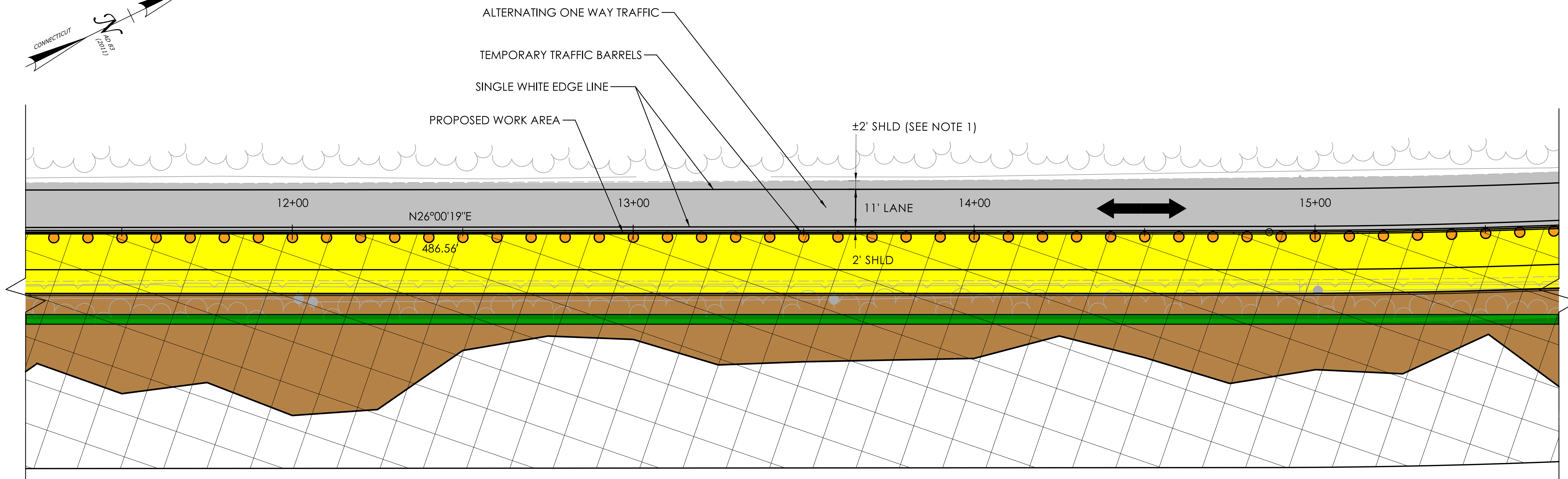
ROADWAY PLAN - DURING CONSTRUCTION
