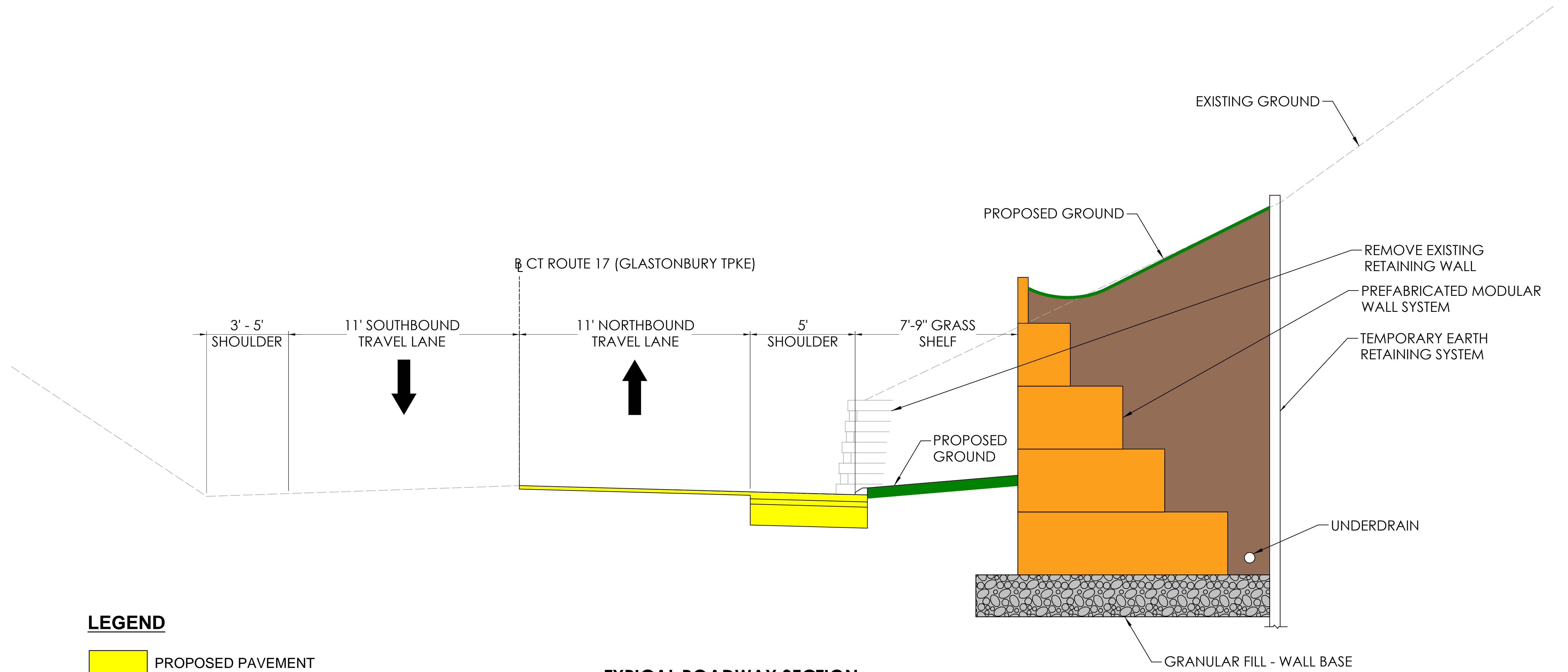
TYPICAL ROADWAY SECTION (LOOKING NORTH ALONG THE ROADWAY)
