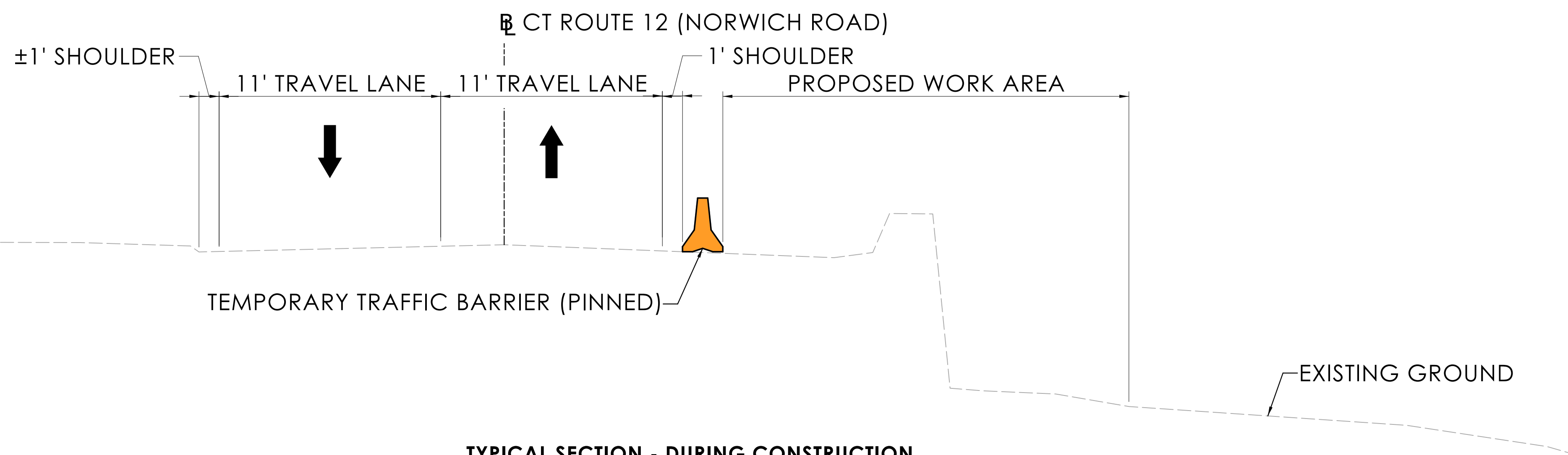
TYPICAL SECTION - DURING CONSTRUCTION (LOOKING SOUTHBOUND)
