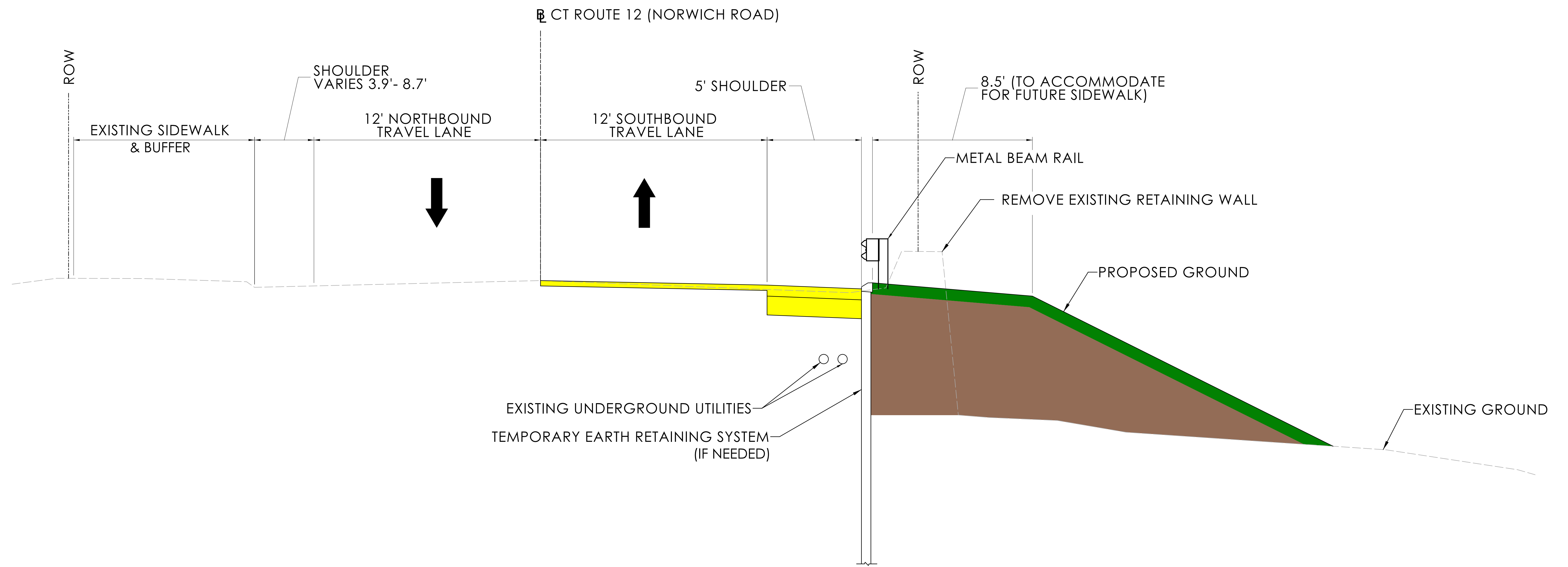
TYPICAL ROADWAY SECTION (LOOKING SOUTHBOUND)
