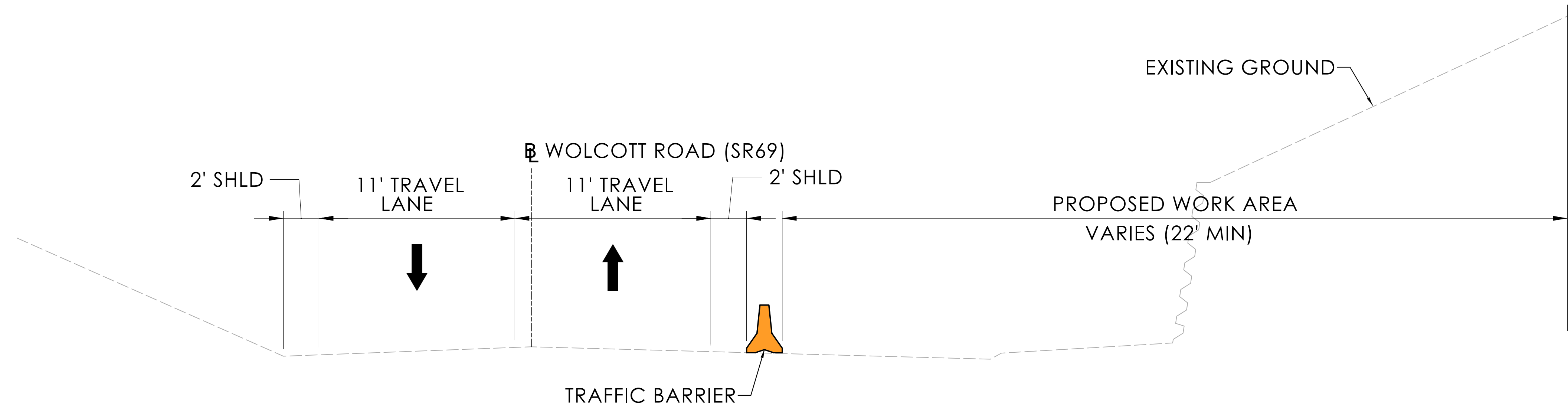
TYPICAL SECTION - DURING CONSTRUCTION (LOOKING NORTHBOUND ALONG ROADWAY)
