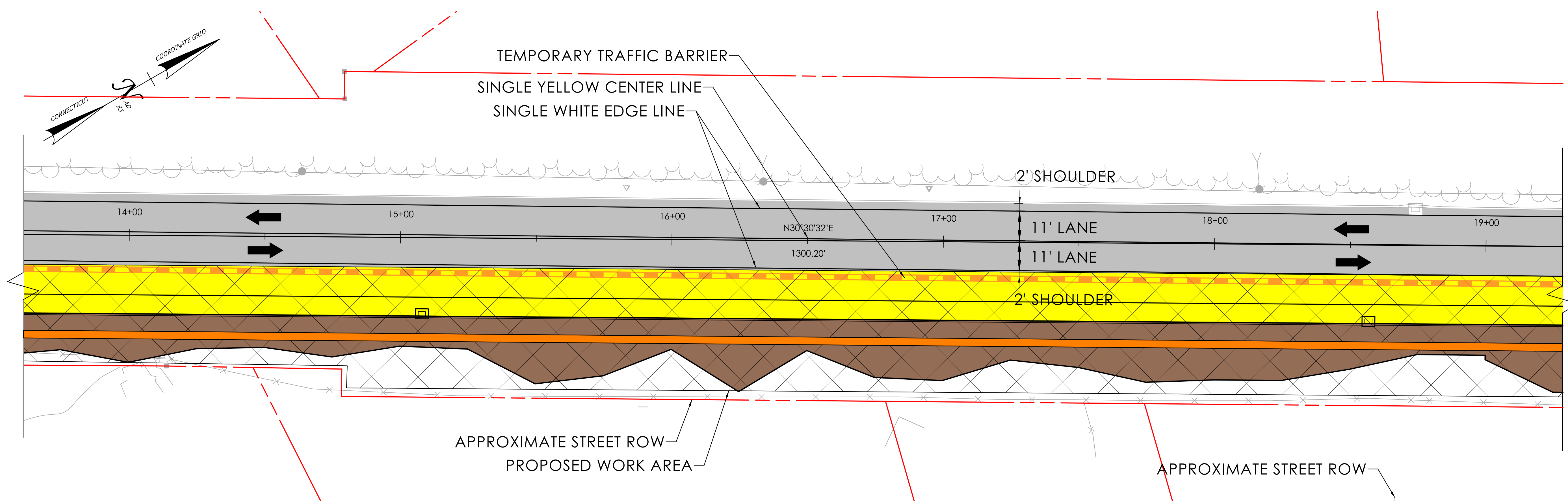
ROADWAY PLAN - DURING CONSTRUCTION
