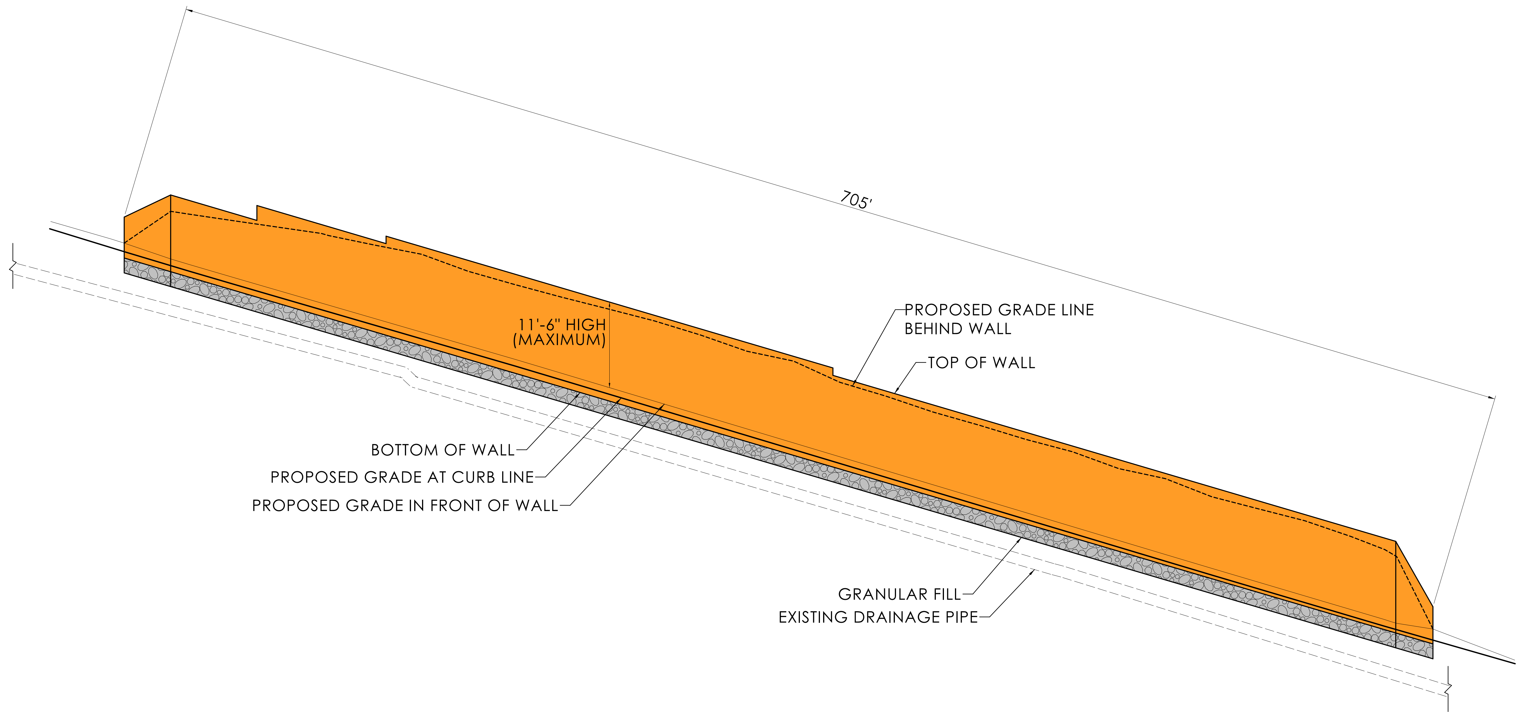
RW-166-069-001 - ELEVATION VIEW (LOOKING AT FACE OF WALL)
