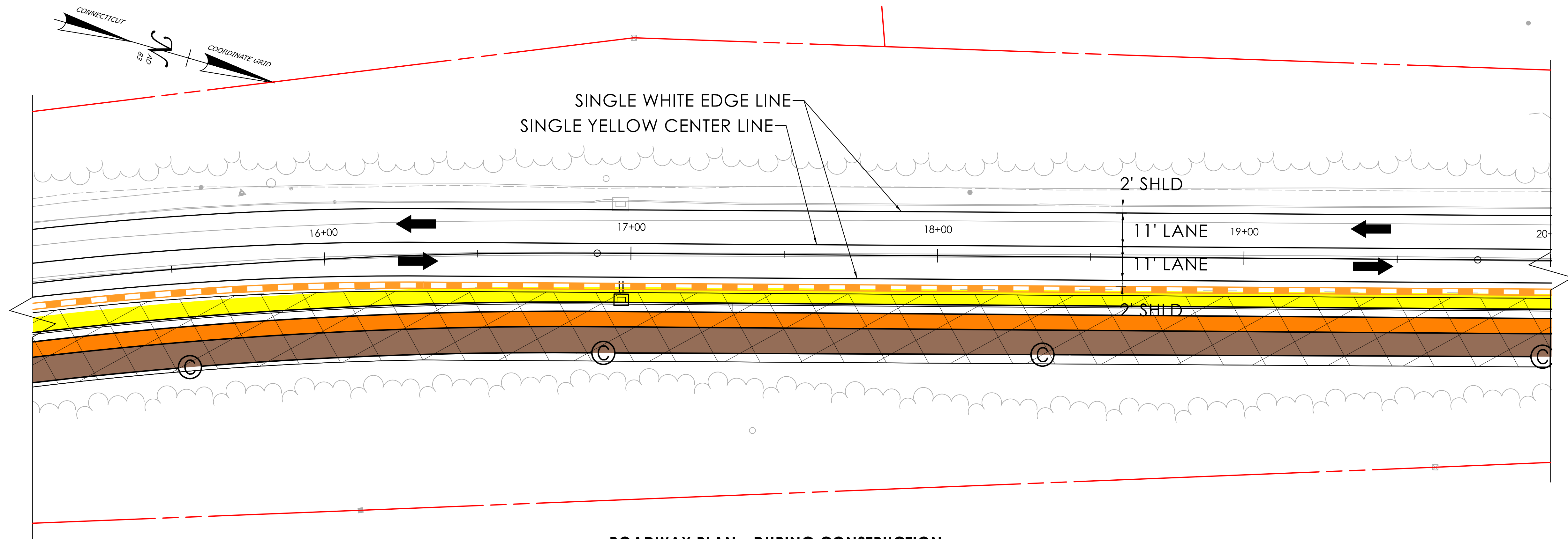
ROADWAY PLAN - DURING CONSTRUCTION
