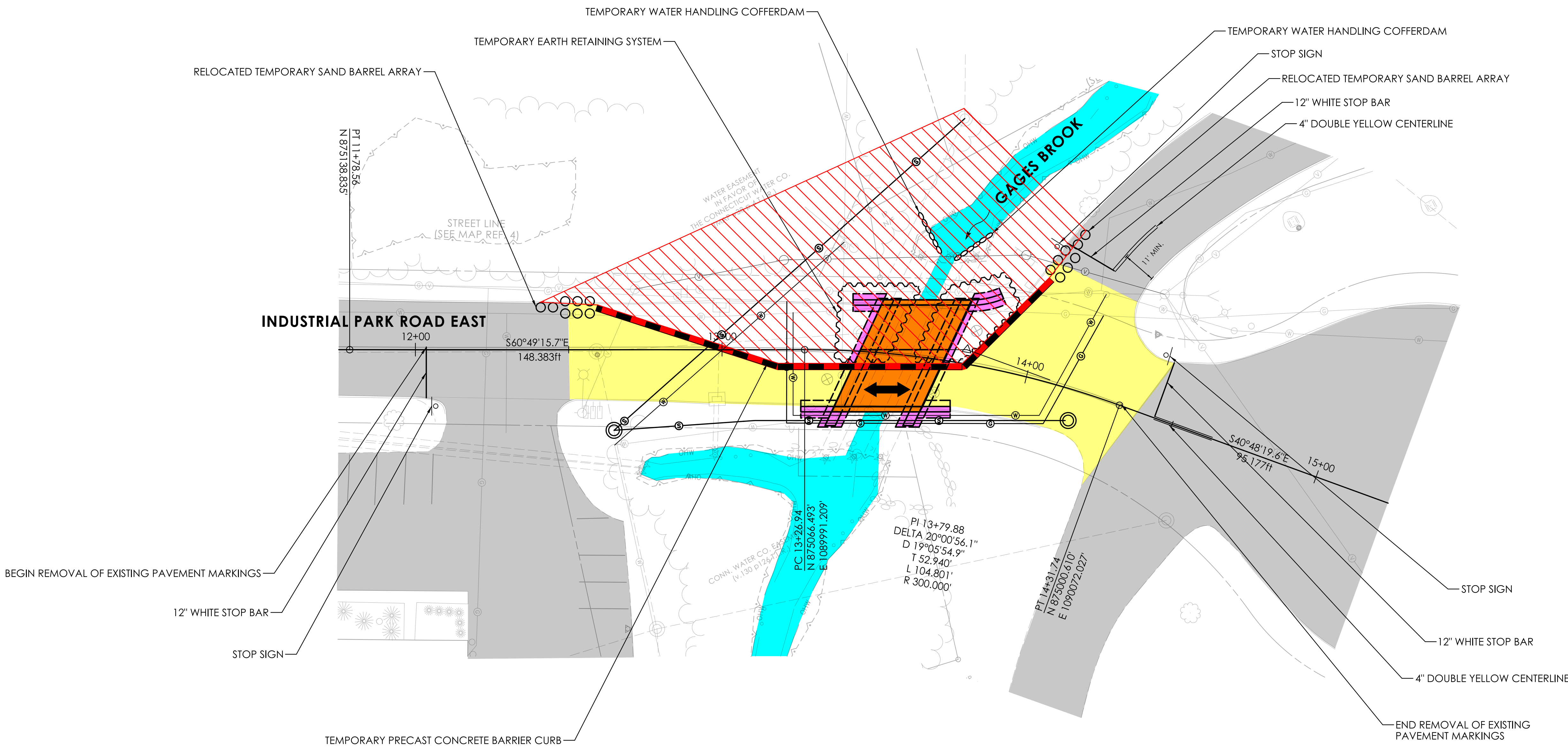
STAGE 2 PLAN
