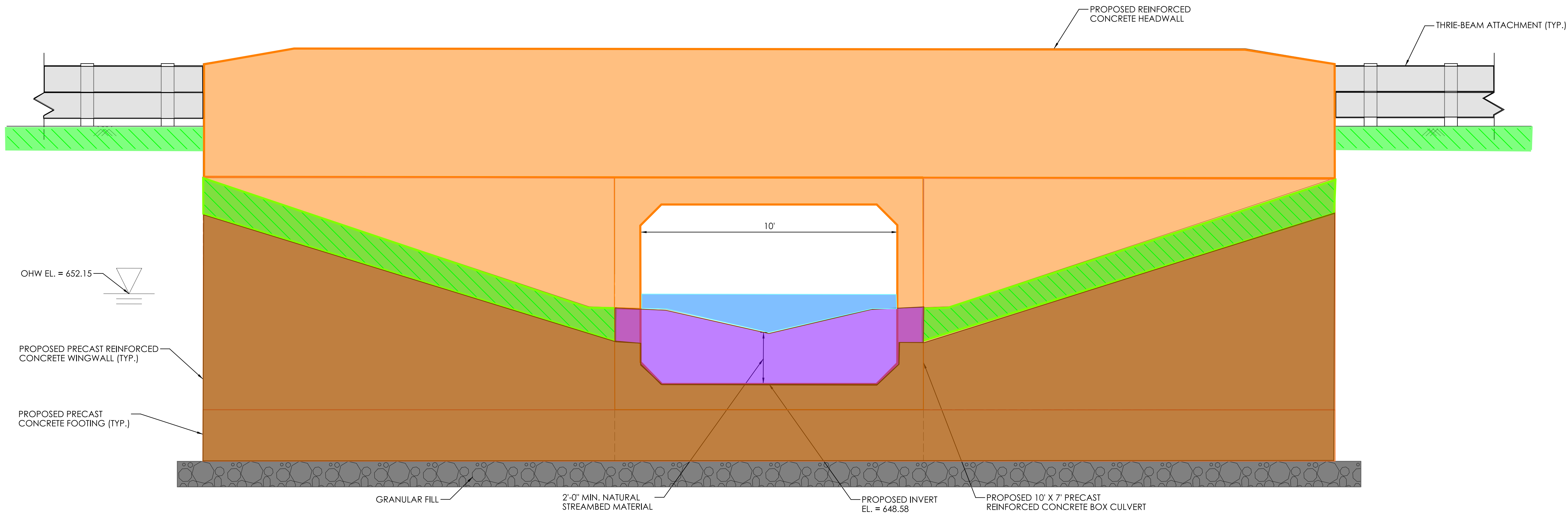
UPSTREAM ELEVATION
