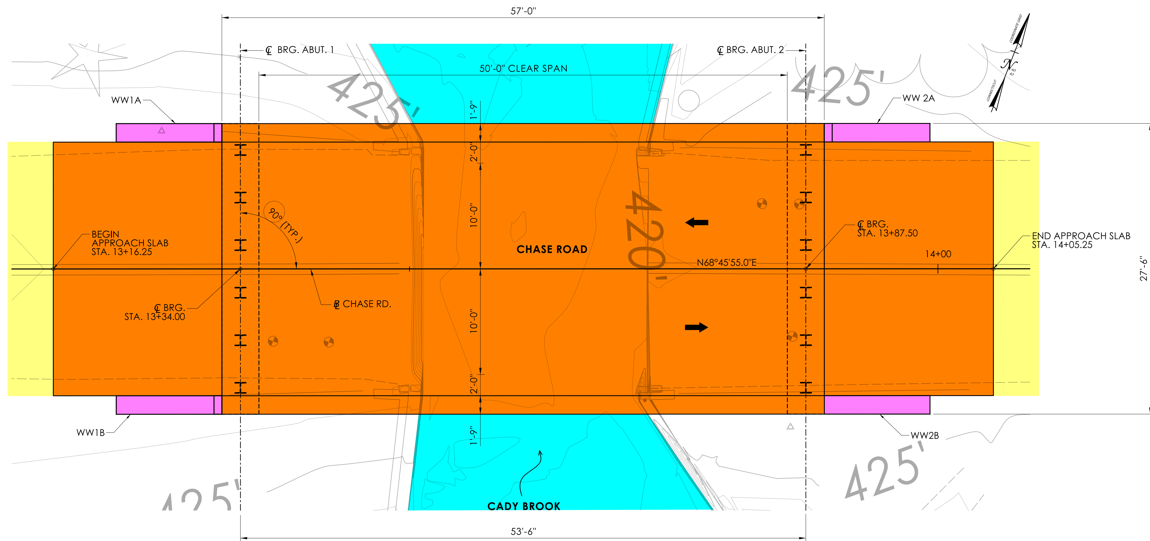
PLAN SCALE: 3/16" = 1'-0"
