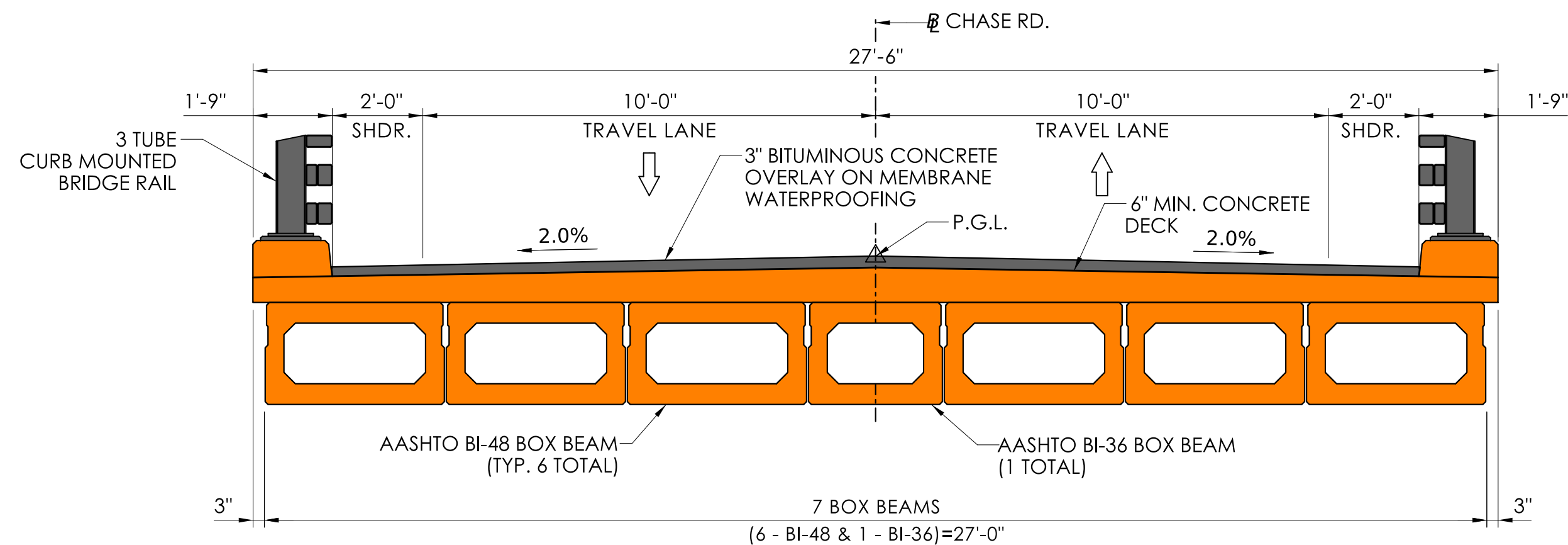
TYPICAL SECTION SCALE: 3/8" = 1'-0"
