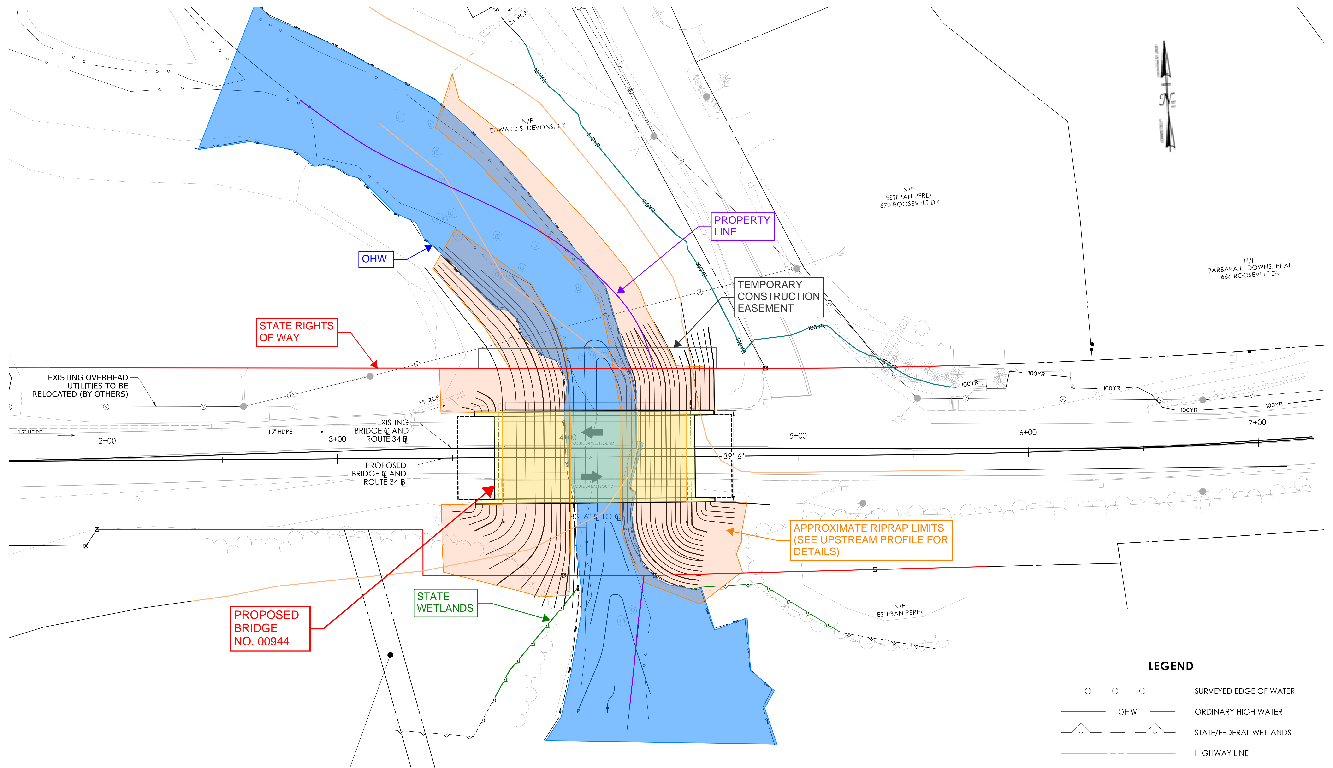
GENERAL PLAN
