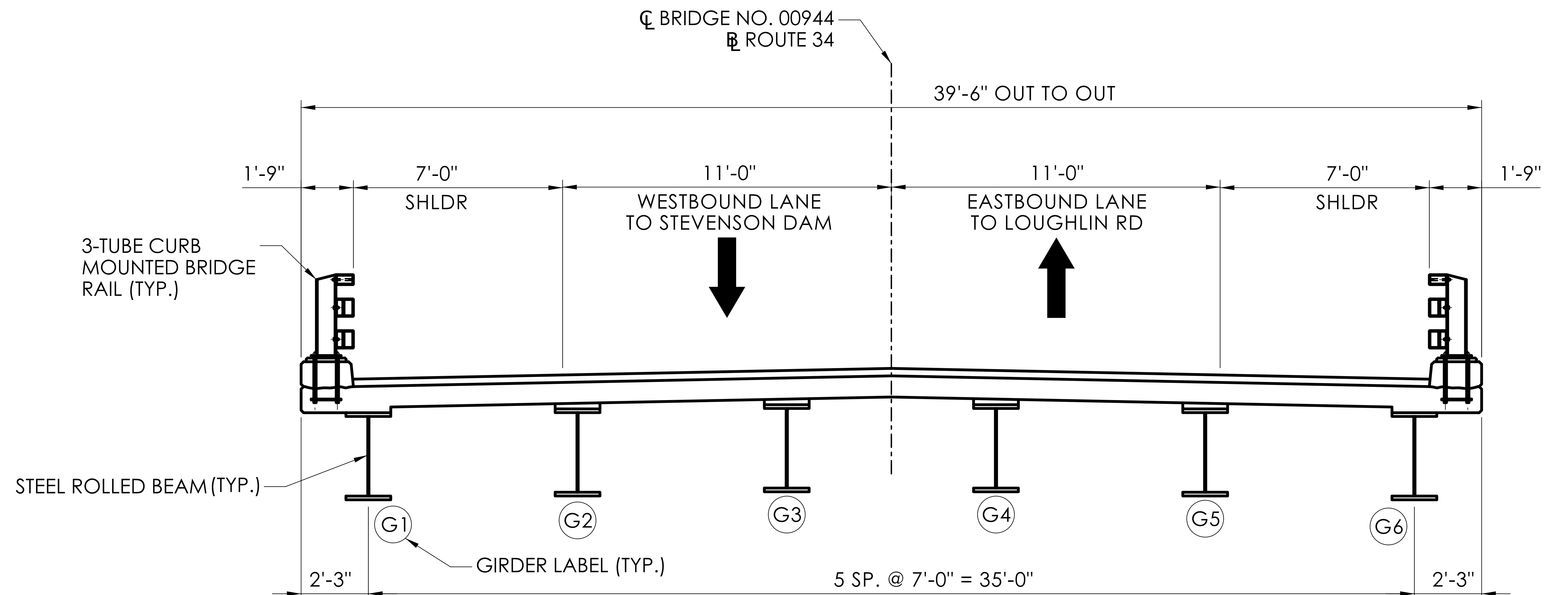
TYPICAL BRIDGE SECTION
