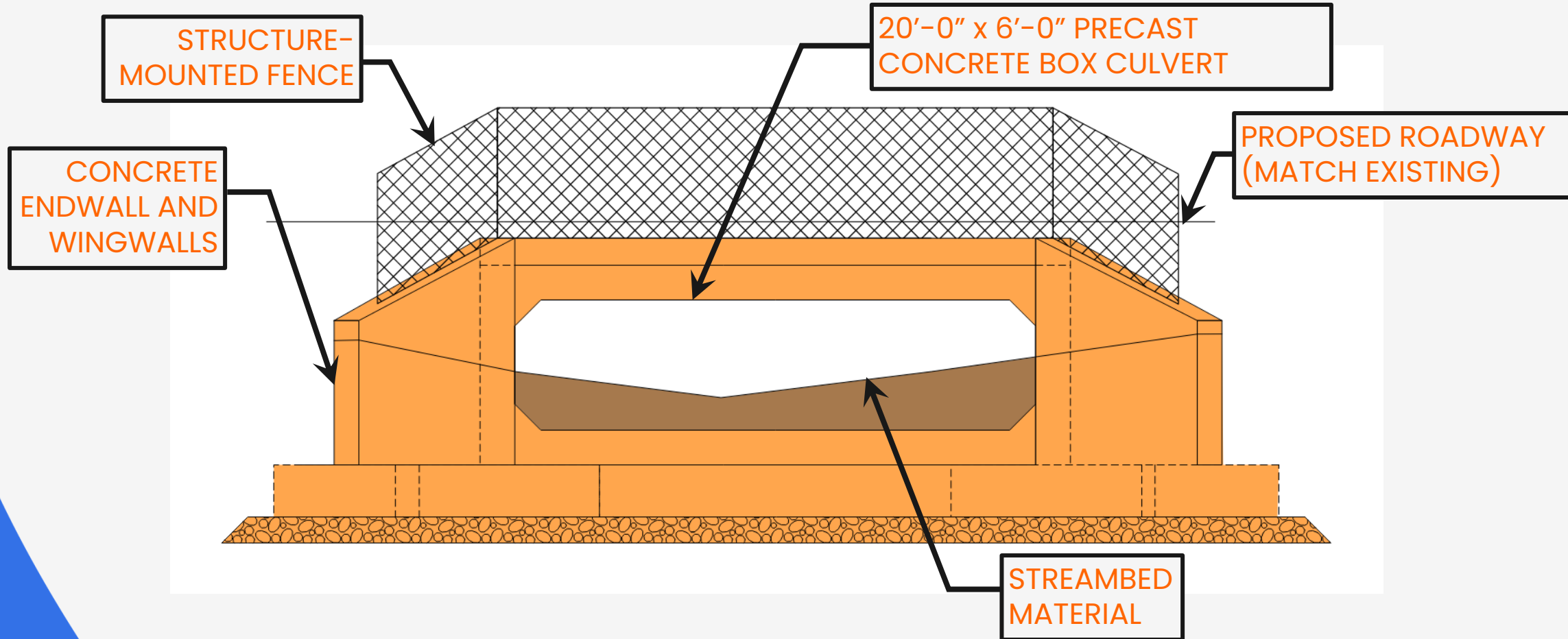
INLET ELEVATION
