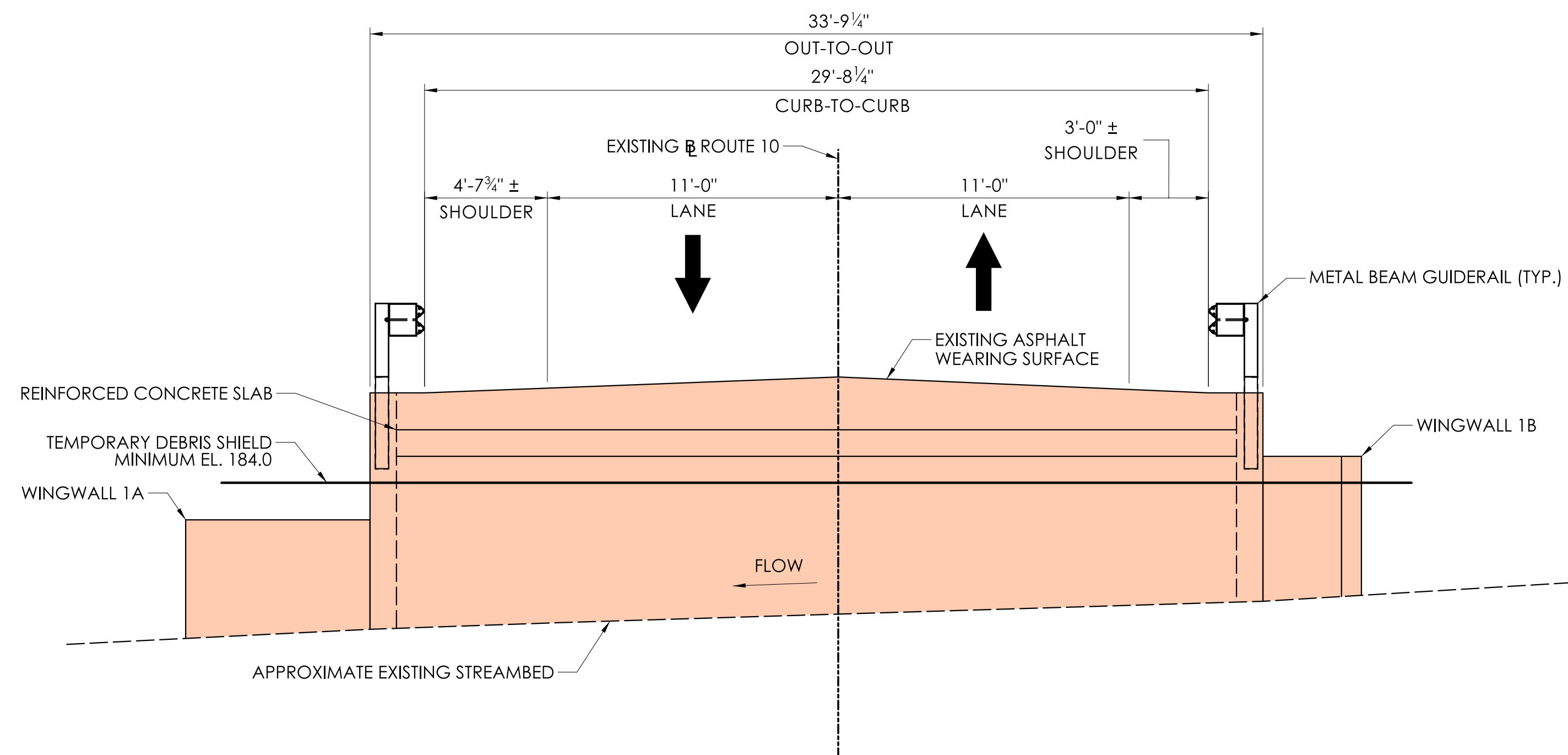
EXISTING CROSS SECTION SCALE: 1/4"=1'-0"
