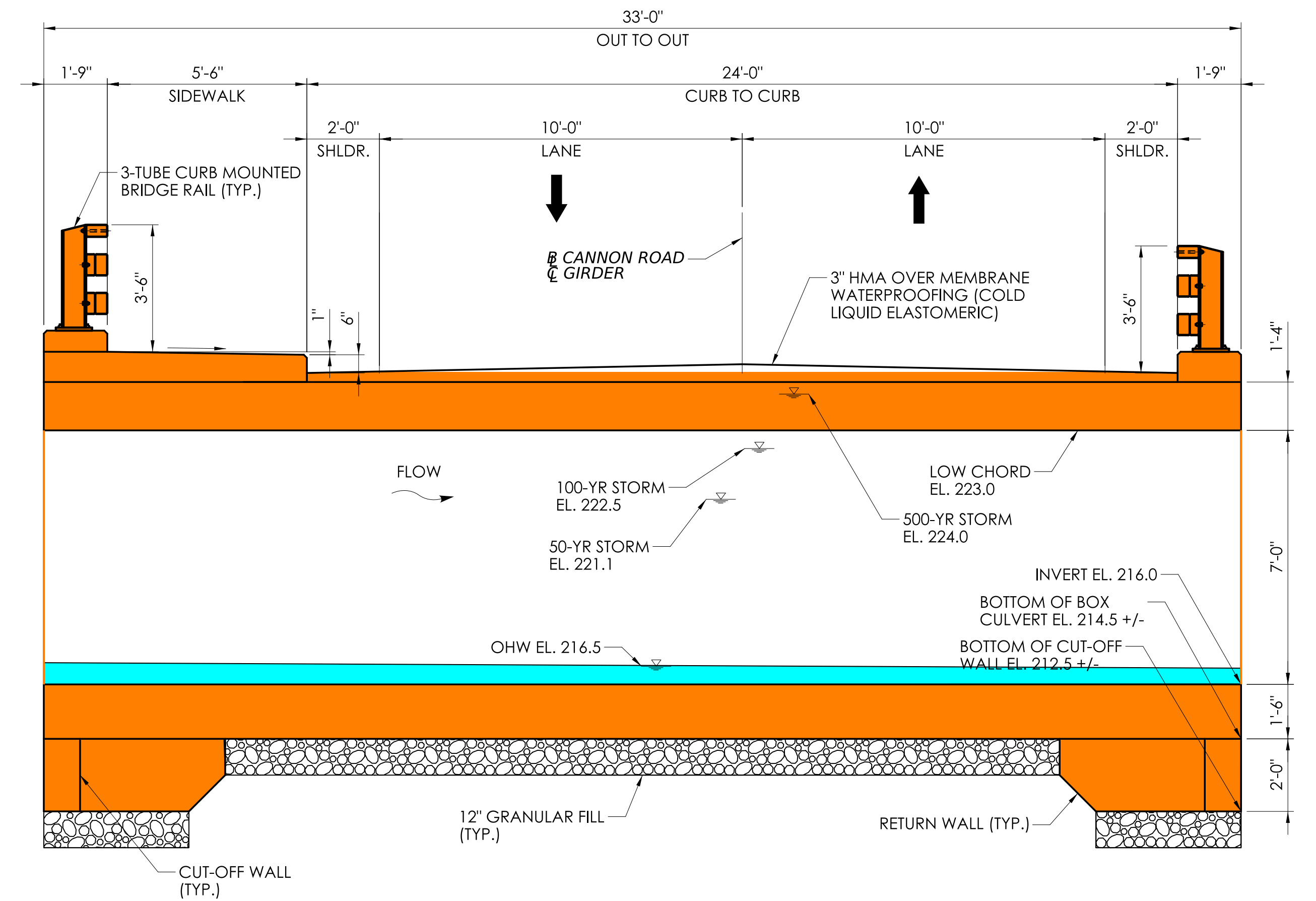
PROPOSED PRECAST CONCRETE BOX CULVERT SECTION (LOOKING EAST) SCALE: 3/8" = 1'-0"
