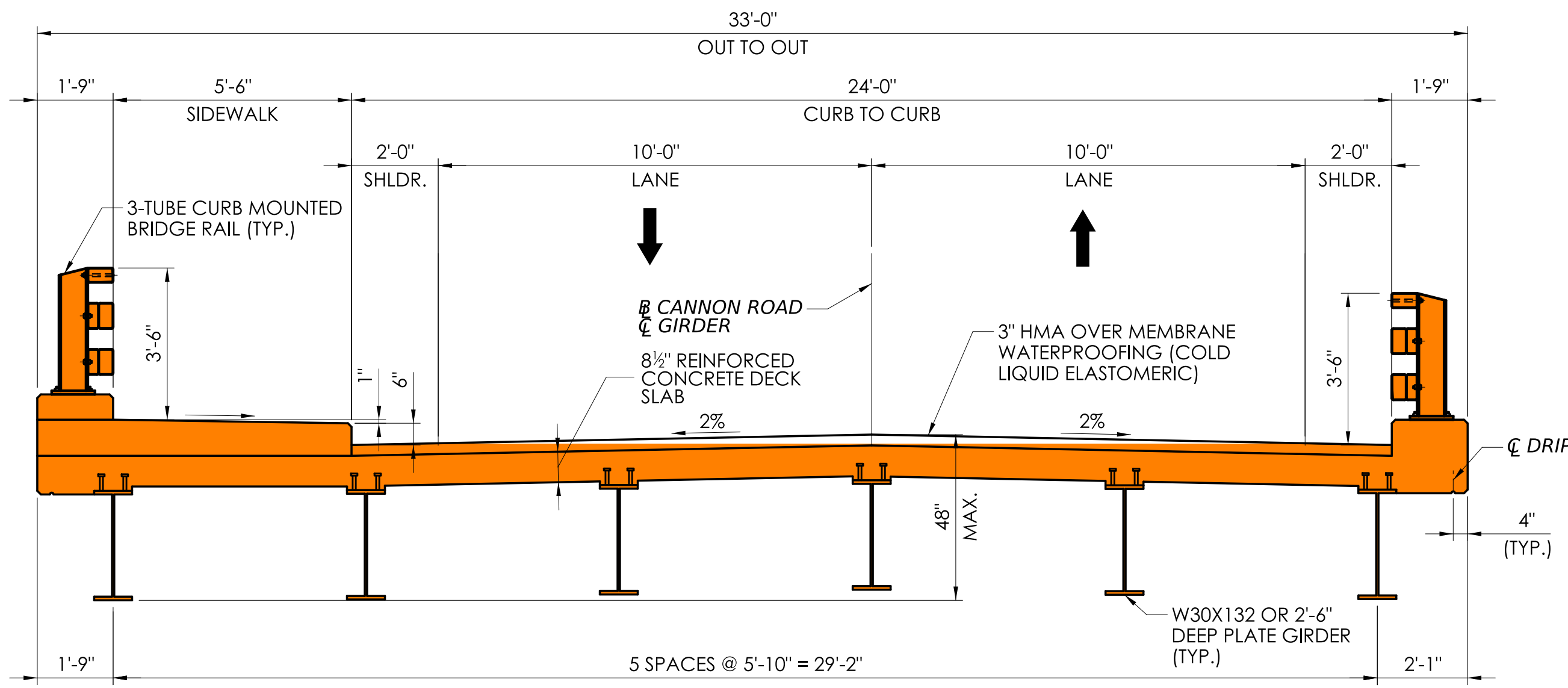
PROPOSED STEEL BEAM BRIDGE SECTION (LOOKING EAST) SCALE: 3/8" = 1'-0"
