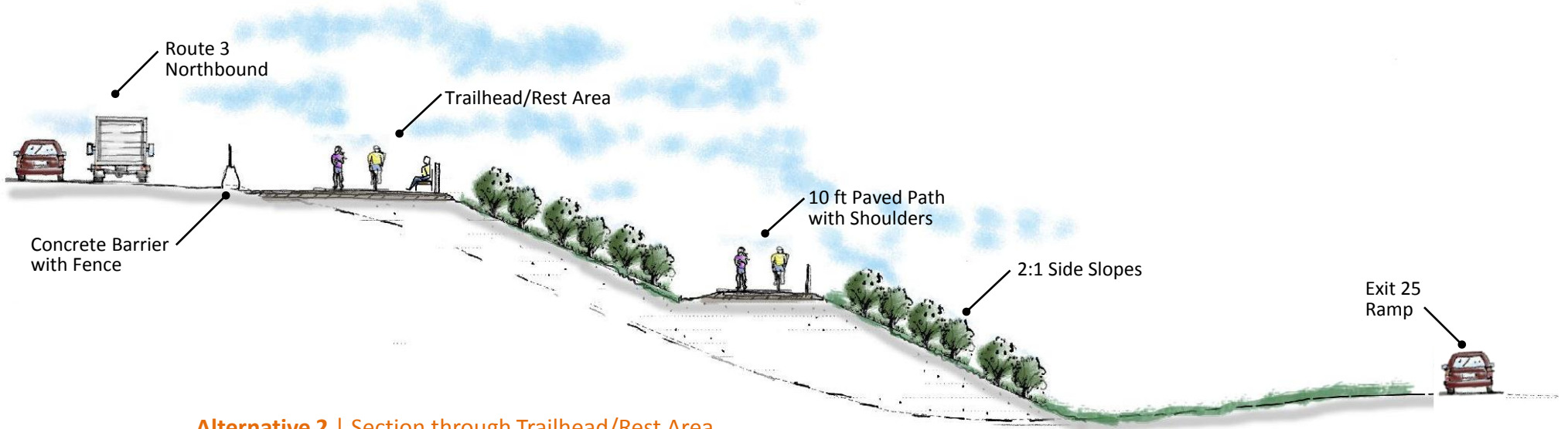
Alternative 2 | Section through Trailhead/Rest Area (looking in northbound direction)
