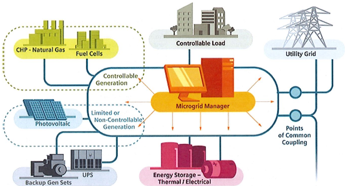
Figure 63: Diagram of a Microgrid
