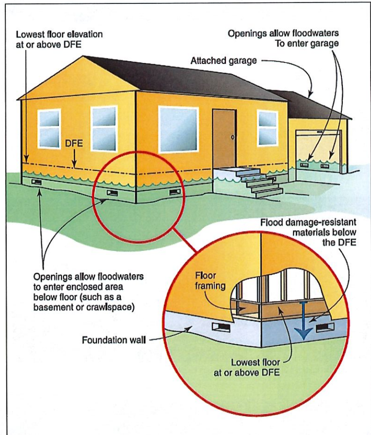
Figure 55: Wet Floodproofing Strategies
