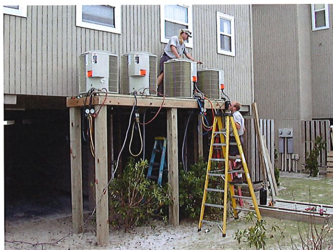
Figure 59: Example of Protecting and Elevating Critical Equipment
