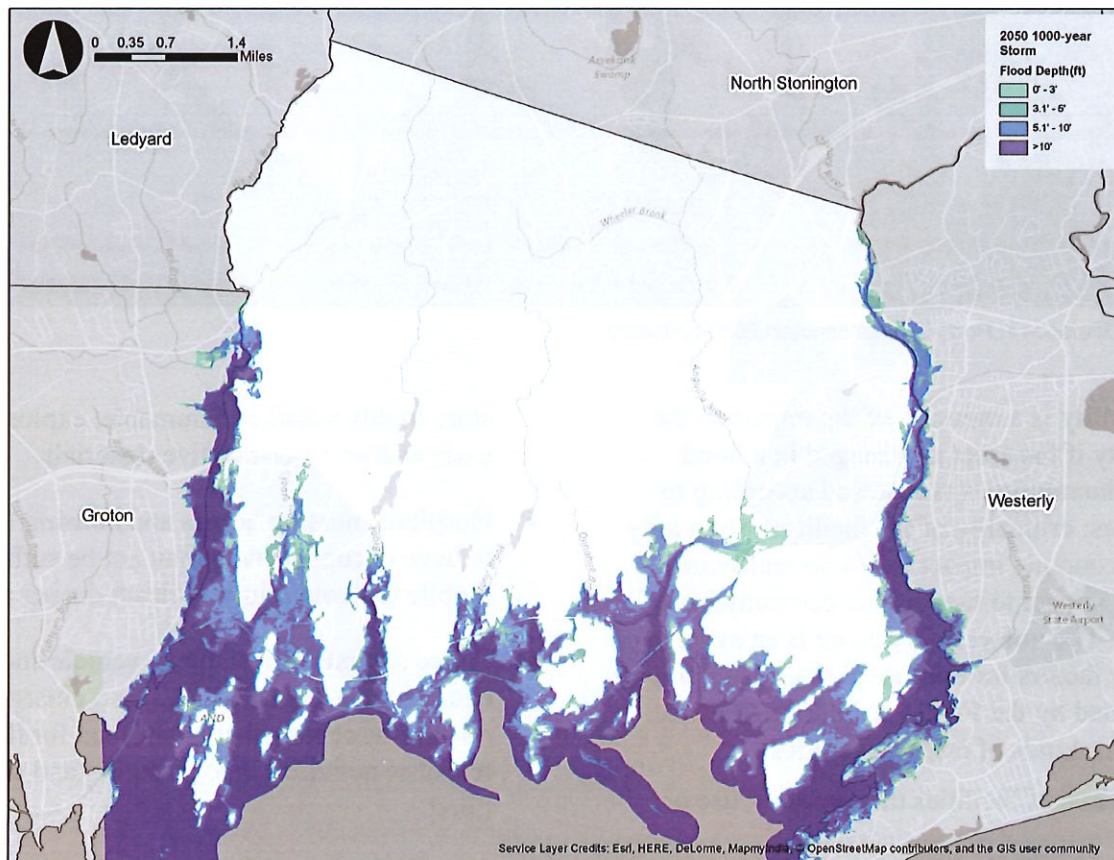
Figure 17: Estimated Flood Depths for a 1000-year Storm Event (0.1% Annual Chance) in 2050
