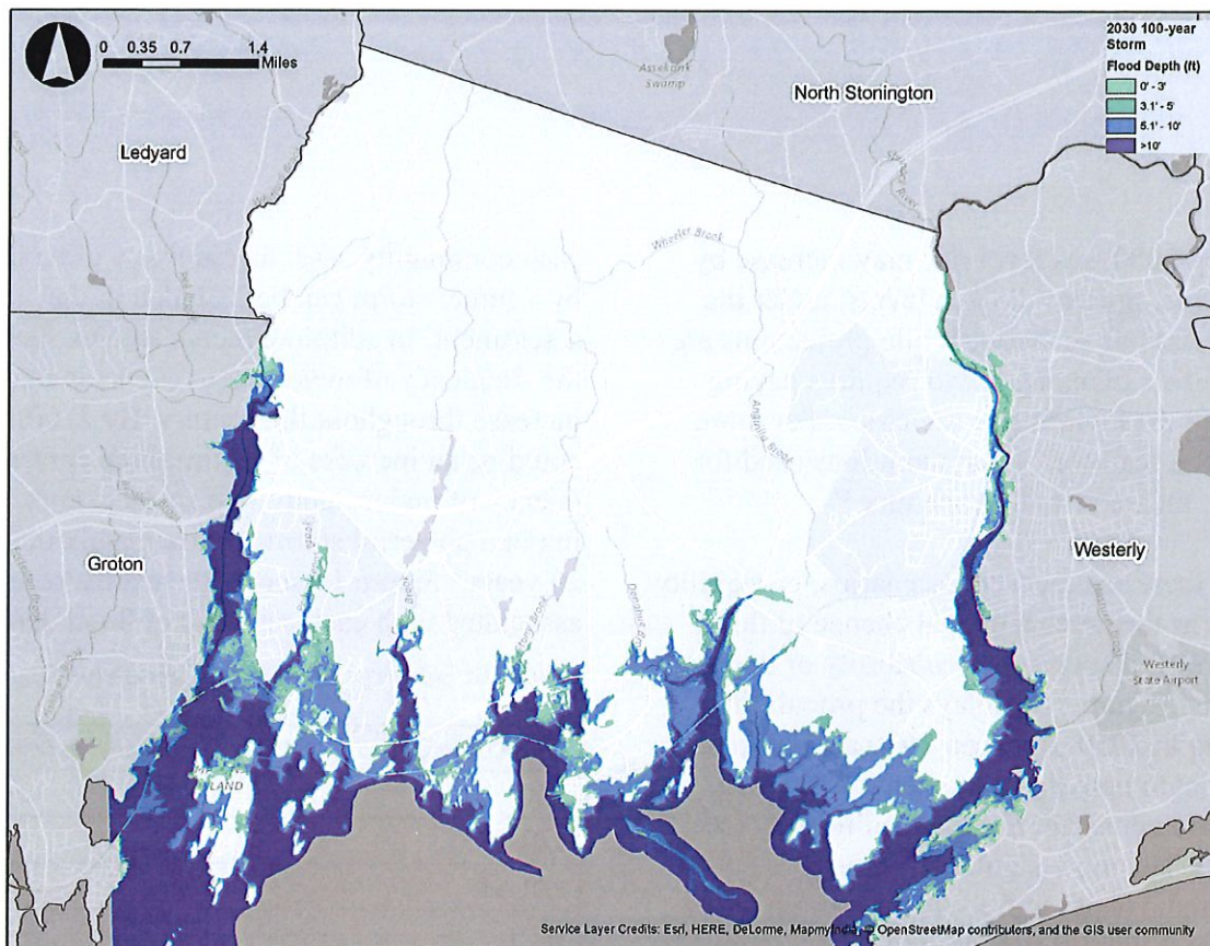
Figure 14: Estimated Flood Depths for a 100-year Storm Event (1% Annual Chance of Flooding) in 2030
