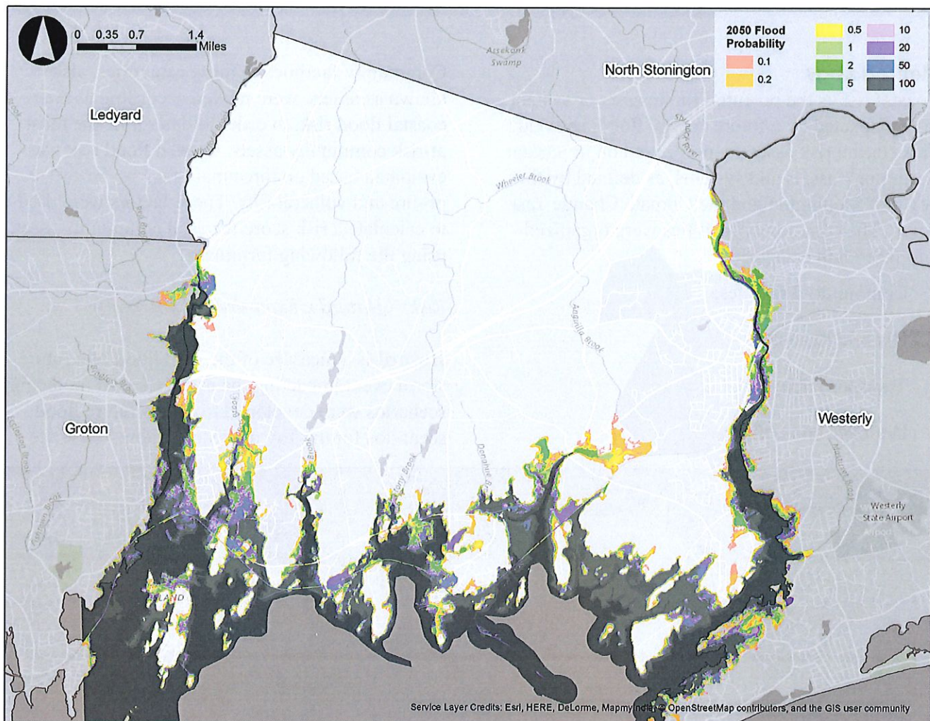
Figure 11: 2050 Flood Probability in Stonington, CT
