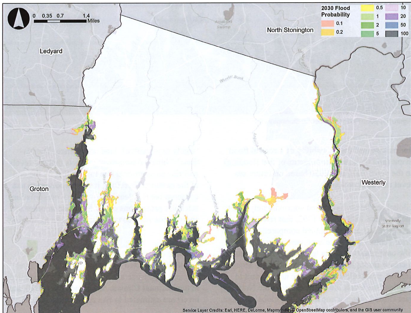
Figure 10: 2030 Flood Probability in Stonington, CT
