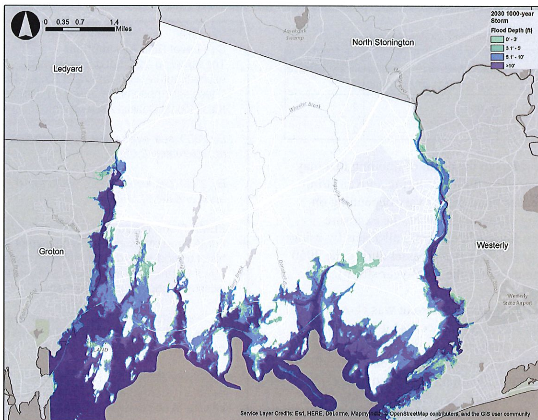
Figure 15: Estimated Flood Depths for a 1000-year Storm Event (0.1% Annual Chance) in 2030
