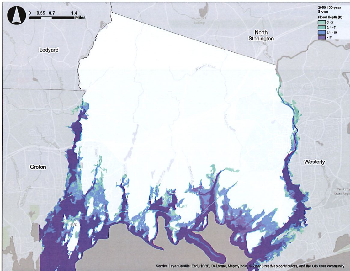
Figure 16: Estimated Flood Depths for a 100-year Storm Event (1% Annual Chance) in 2050
