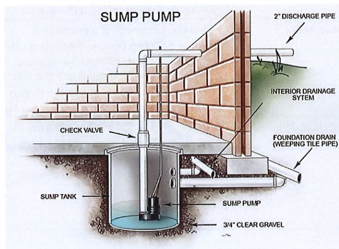
Figure 62: Diagram of a Sump Pump
