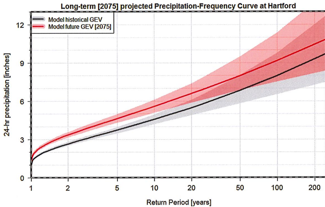
Figure 3-15: As in Fig. 3-14 except for the 2075 period.
