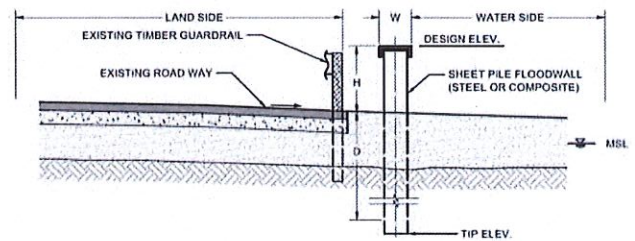
ROAD SIDE SHEET PILE FLOODWALL - CONCEPTUAL
