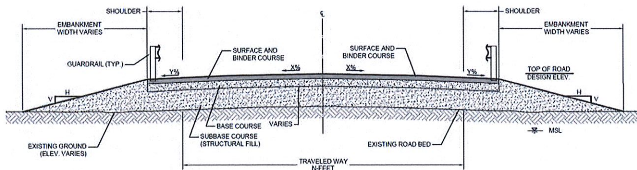
RAISED ROAD WAY
