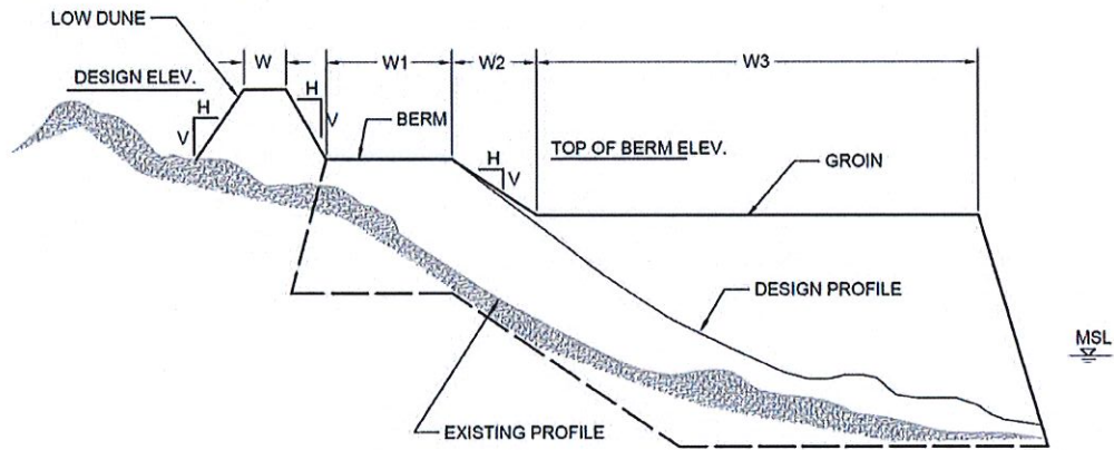
BEACH NOURISHMENT - CONCEPTUAL
