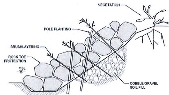
VEGETATED REVETMENT - CONCEPTUAL
