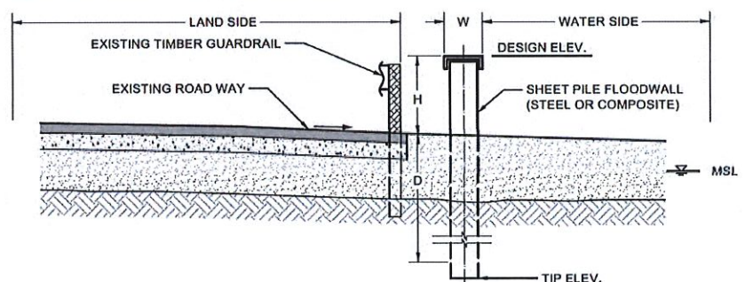
ROAD SIDE SHEET PILE FLOODWALL - CONCEPTUAL
