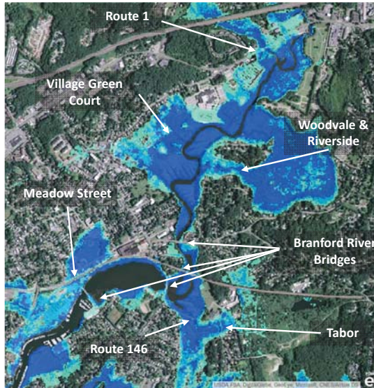
Present Day Category 2 Storm
