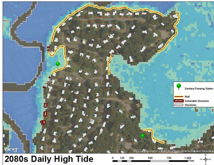
Floodwall system during projected 2080s high tide
