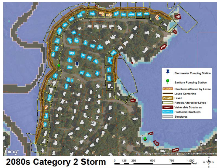
2080s Category 2 Storm Levee system during projected 2080s Category 2 storm
