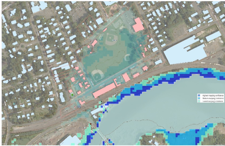
Open Railroad Underpass 2050s Highest High Tide Water elevation projected at approximately 5.8 feet (NAVD83). Meadow St. Neighborhood (lighter area) will be flooded if high water overtops Indian Neck Rd. at location indicated.
