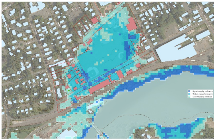
Open Railroad Underpass 2080s Highest High Tide Water elevation projected at approximately 4.7 feet (NAVD83). High water is expected to overtop Indian Neck Road and flood Meadow Street Neighborhood.
