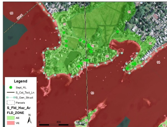
Summer Island Point FEMA transect and DFIRM
