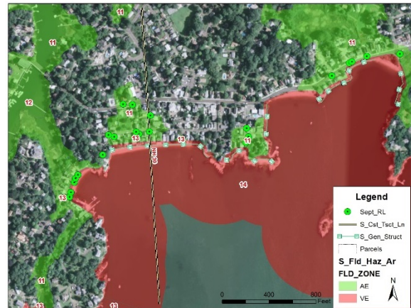
Short Beach FEMA transect and DFIRM
