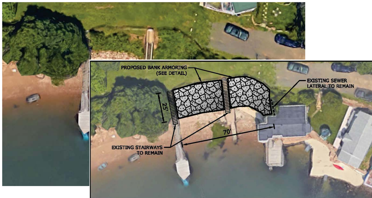
SHORELINE STABILIZATION - PLAN VIEW
