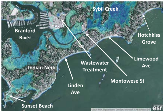
2020 Daily Inundation
