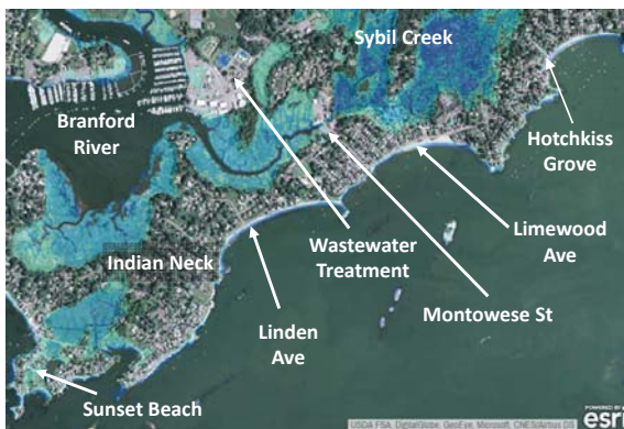
2020 Daily Inundation
