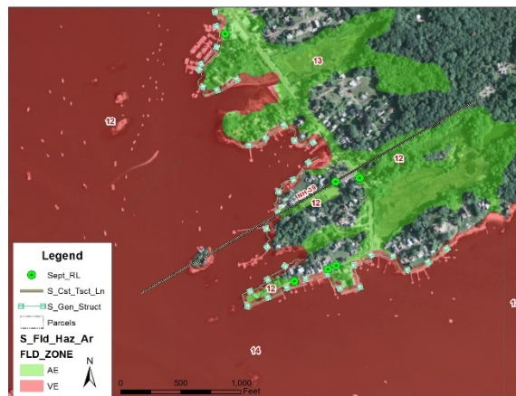
Thimble Island Road FEMA transect and DFIRM
