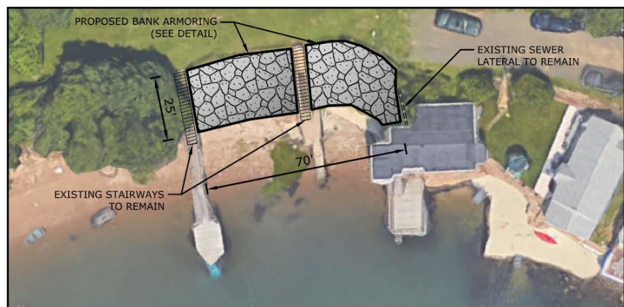
SHORELINE STABILIZATION - PLAN VIEW
