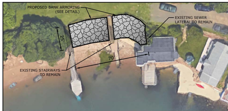
SHORELINE STABILIZATION - PLAN VIEW SCALE 1" = 30'
