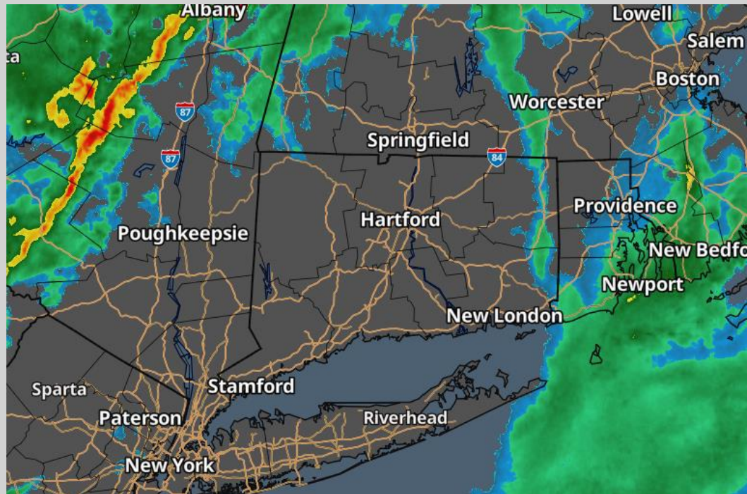
RADAR AS OF 19:45
