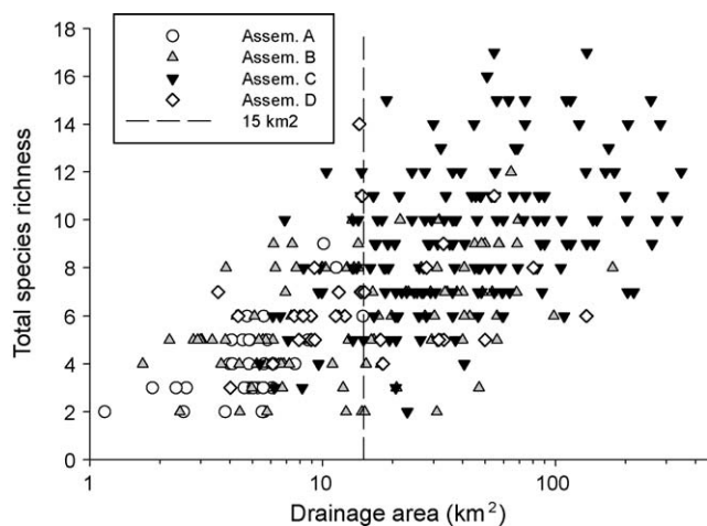
Fig. 1. Relationships between drainage area (km 2 ) and total species richness in 348 Wadeable streams in Connecticut. Assemblage type designation is based on a discriminant function derived from Kanno and Vokoun (2008). Drainage area is on a logarithmic scale.
