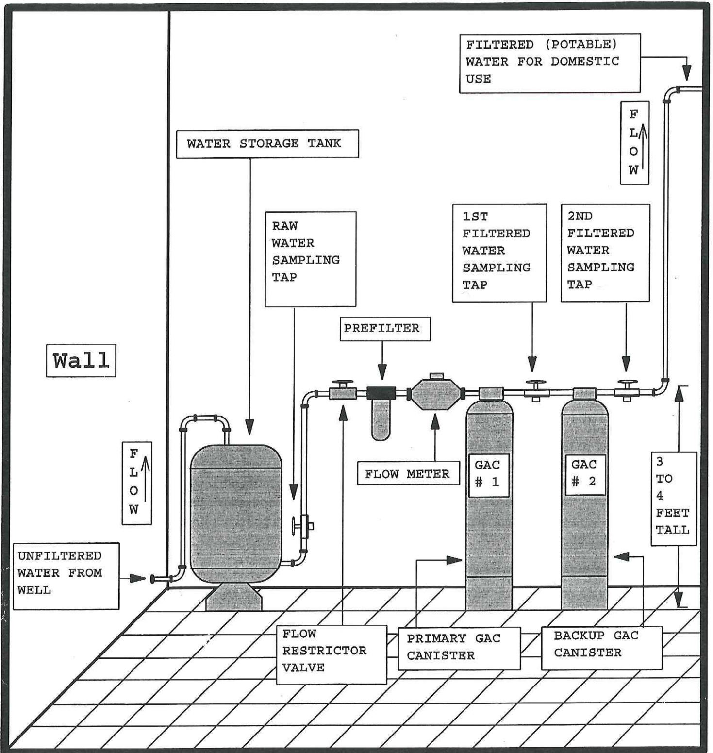
TYPICAL GRANULAR ACTIVATED CARBON (GAC) FILTER SYSTEM
