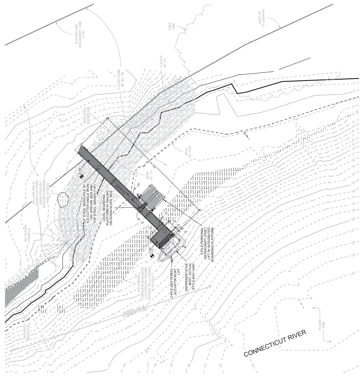
1 PROPOSED DOCK PLAN 1" = 10'-0"
