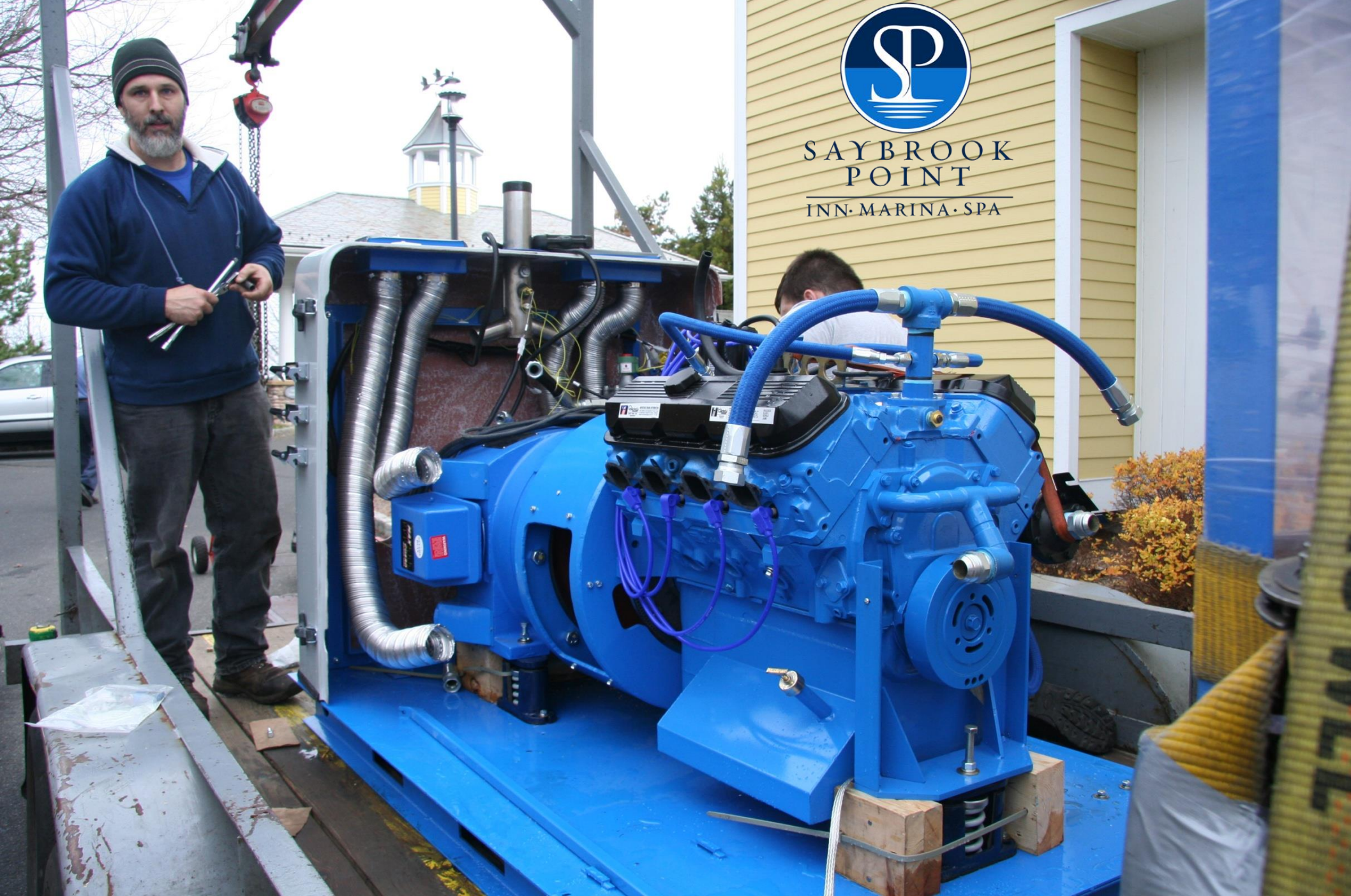
Natural Gas Co-Generation Plant
