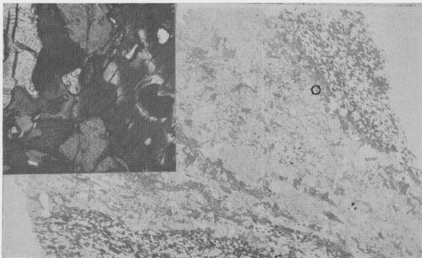
Thin section of epidote amphibolite variety of Hebron gneiss. Enlargement about 20X. Inset is photomicrograph of encircled area, enlargement 50X.
