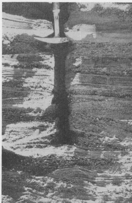
Cross-bedded sand and fine gravel; typical fluvio-glacial material such as covers much of the quadrangle west of the Bolton ridges. Pebbles are predominantly Triassic or quartz with a scattering of small discs of Bolton schist. Photograph of gravel bank on west side of West Street just south of Rockville city line (NW).
