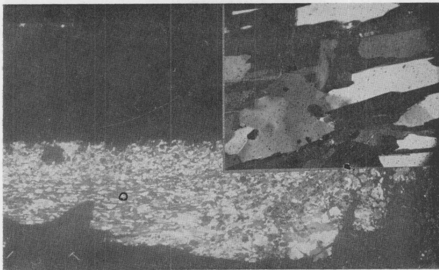
Thin section of Bolton micaceous quartzite. Enlargement about 20X. Inset is photomicrograph of encircled area, enlargement 50X.
