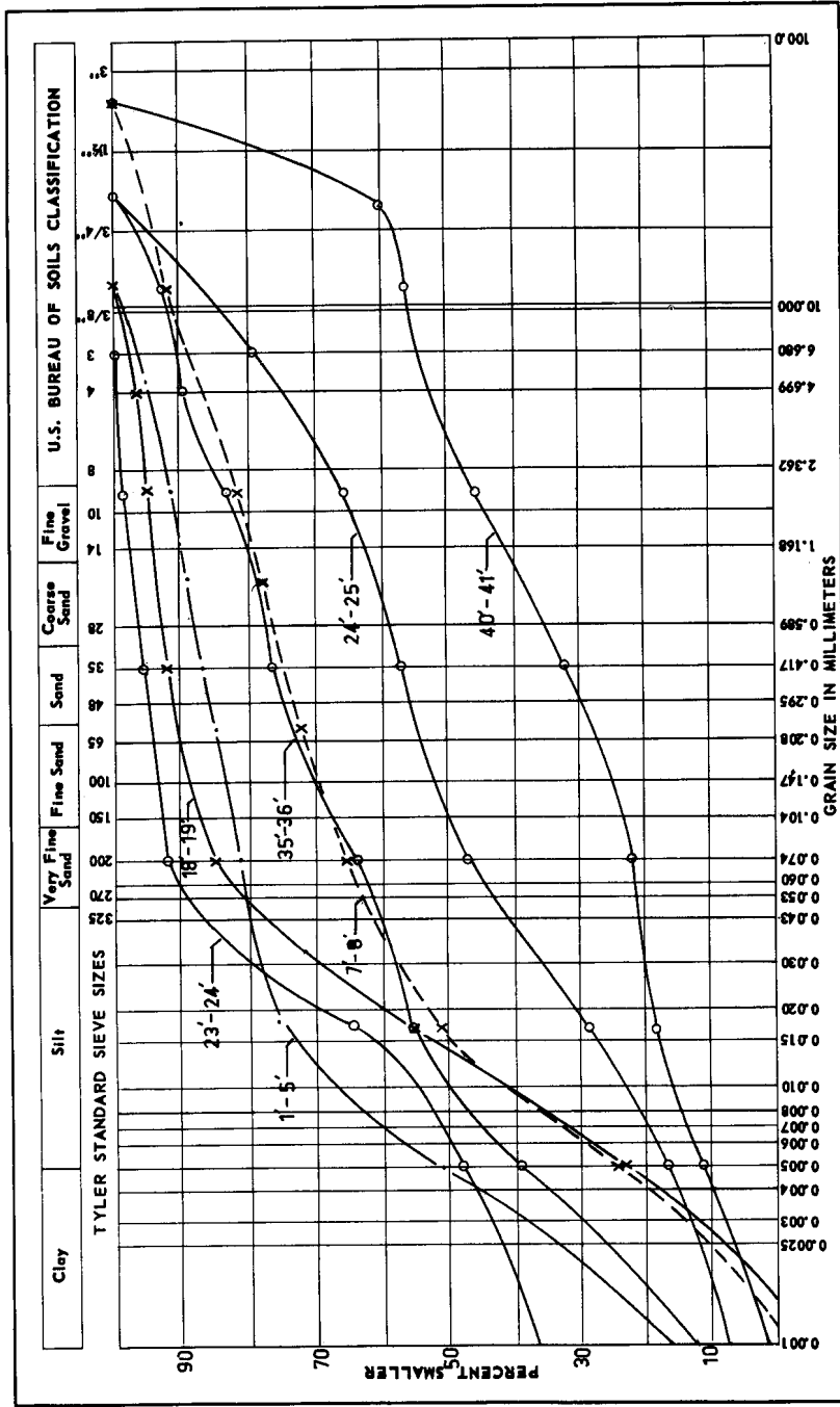
Fig. 7. Cumulative curves of a suite of samples from borehole SD-14. See table 2 for location of samples. Samples are identified by depths in ft in borehole; those from 1 to 25 ft are from a till that overlies varved clays which are at depths of 25 to 30 ft; those from 35 to 41 ft are from the till underlying the varved clay. Analyses supplied by the Connecticut State Highway Department.
