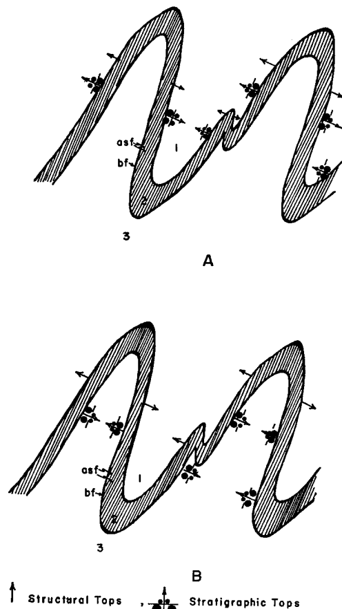
Fig. 3. Profile diagram of a hypothetical series of folds showing the relation between bedding foliation (bf), axial-surface foliation (asf), and graded bedding.
