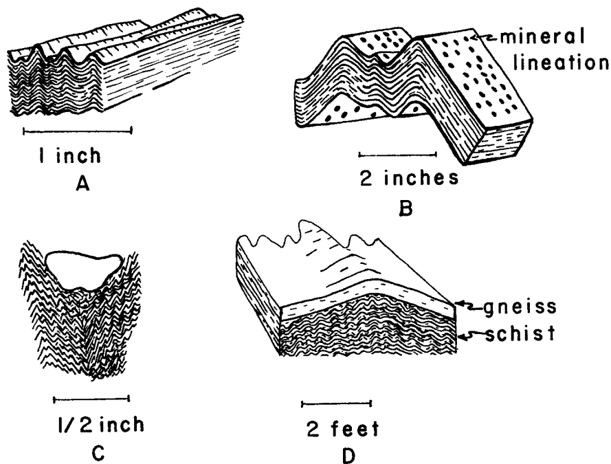
Fig. 9. Crenulate folds. A shows the character of the profile and the fold axis. Mineral lineation deformed by crenulate folds is shown in B . C shows the change in sense of rotation around a quartz porphyroblast. Contrasting fold styles in schist and gneiss are shown in D .
